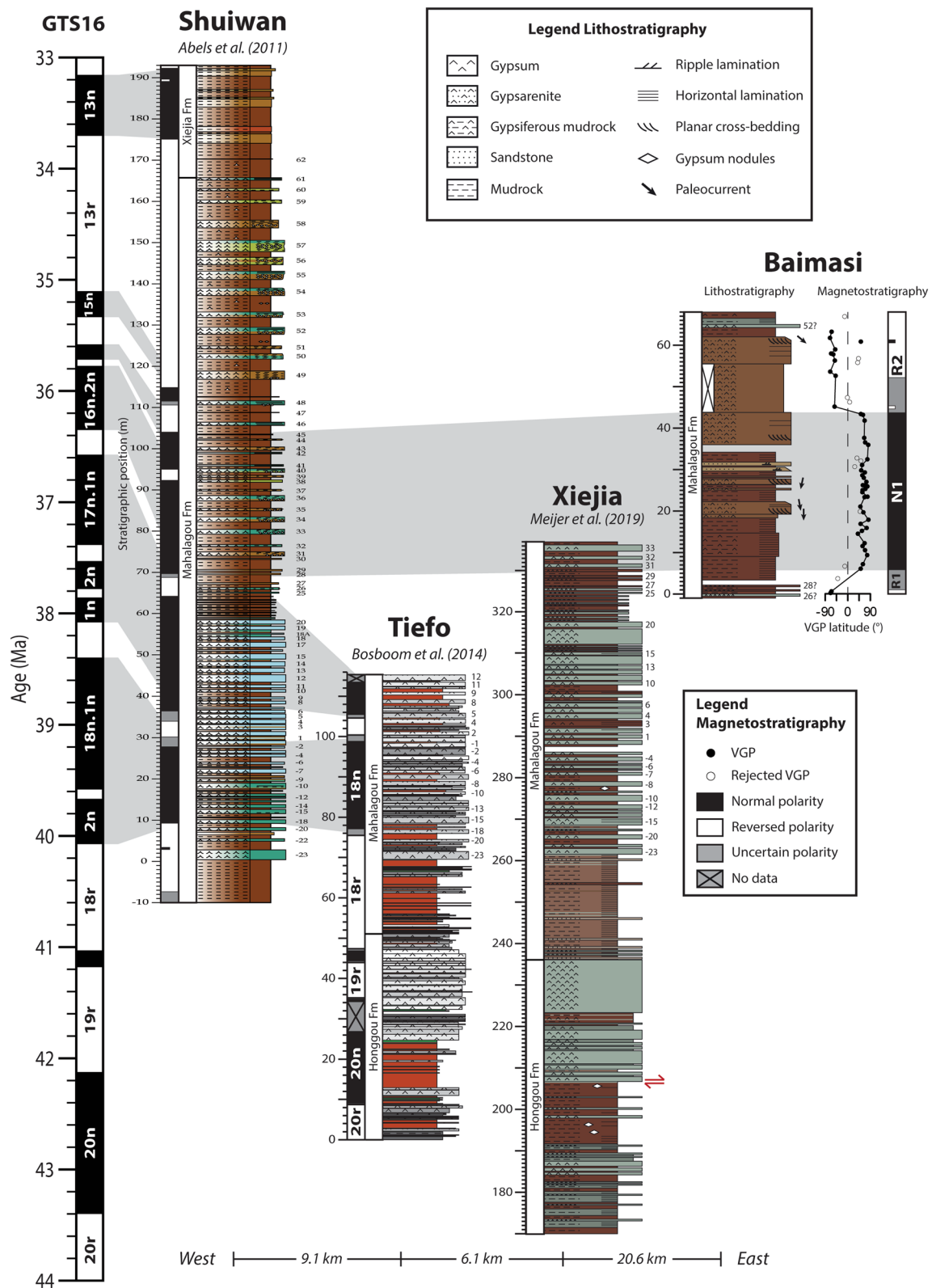
Figure 4. Lithostratigraphic and magnetostratigraphic correlations between the Shuiwan (Abels et al., 2011), Tiedo (Bosboom et al., 2014), Xiejia (Meijer et al., 2019) and Baimasi sections and the GTS16 (Ogg et al., 2016).
