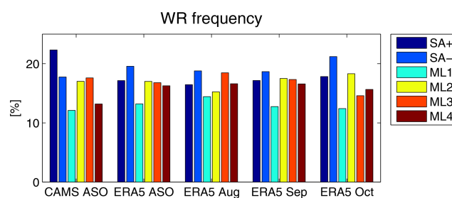
Figure 7. WR frequency in CAMS (computed in the period 2003–2017) and ERA5 (computed in the period 1981–2020) classifications.
