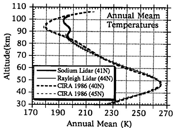
Fig. 2. Annual mean temperatures from harmonic analysis. The broad and thin solid curves are deduced from Na lidar (83 - 103 km) and Rayleigh lidar (30 - 87 km), respectively. The broad and thin dotted curves are from CIRA 1986 for 40°N and 45°N.
