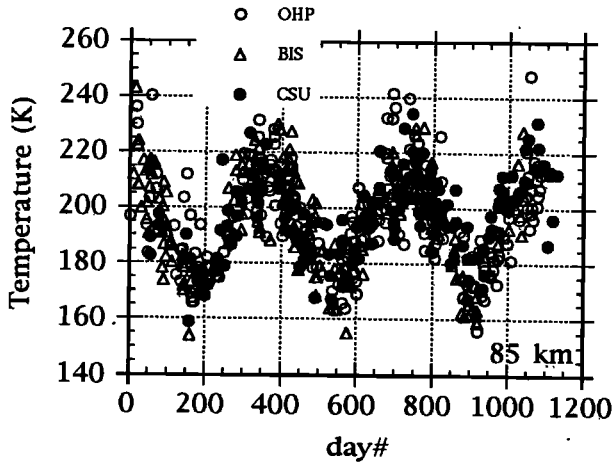
Fig. 1. Measured nightly averaged temperatures at 85 km at FC, OHP and BIS from 1991 to 1993. Similar agreements hold throughout the 82-90 km range.
