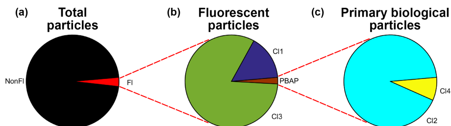
Figure 1. The relative proportions of the non-fluorescent, N_{\text{NonFL}} , and fluorescent, N_{\text{FL}} , aerosol populations (a); the cluster solution concentrations, Cluster 1 (C11, moderately fluorescent), C13 (very weakly fluorescent), and PBAP (strongly fluorescent, b); PBAP here consists of the two clusters, C12 and C14 (c).
