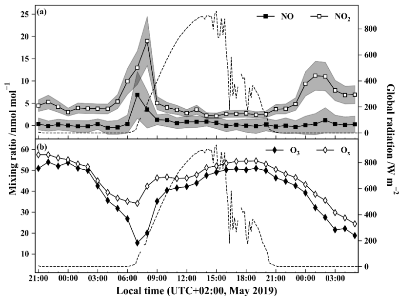
Figure 2: Temporal evolution of (a) NO (closed squares) and NO 2 (open squares) at the sampling site (the grey envelopes represent ± 1σ variations over 1 hour) and of (b) O 3 (close diamonds) and O x (= O 3 + NO 2 ; open diamonds) at the air quality station during sampling. Markers represent for (a) the hourly mean derived from 1-min measurements and for (b) hourly mean provided by the air quality station. Global solar radiation measured at 200 meters from the sampling site is represented by dashed lines.
