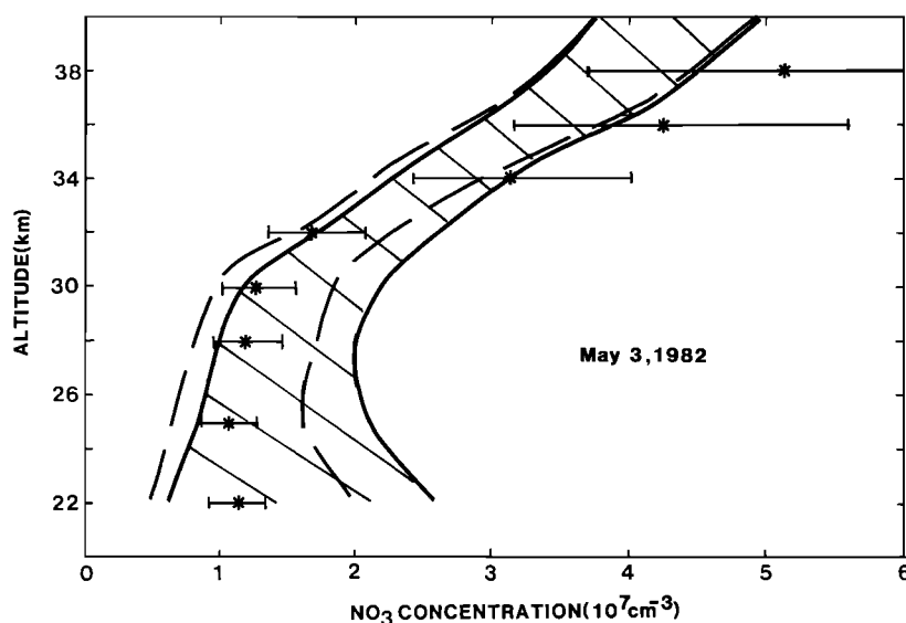
Fig. 5. Same as Figure 3, except for May 3, 1982, at 0330 LT.
