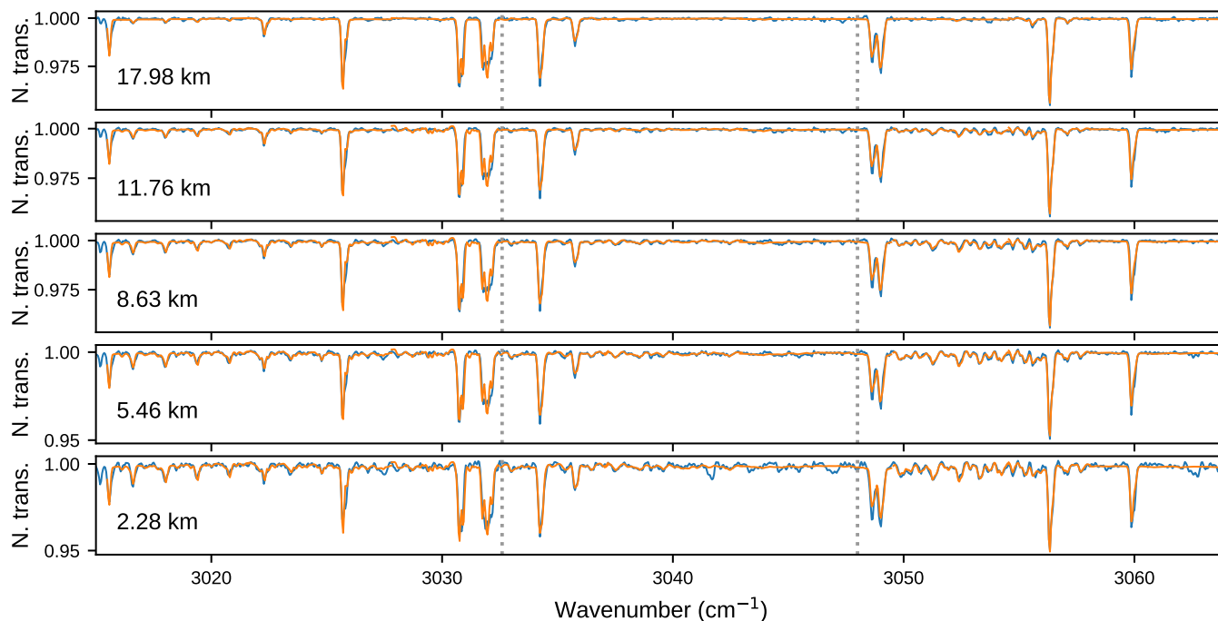
Fig. 2. Same as Fig. 1b, except at a range of altitudes.
