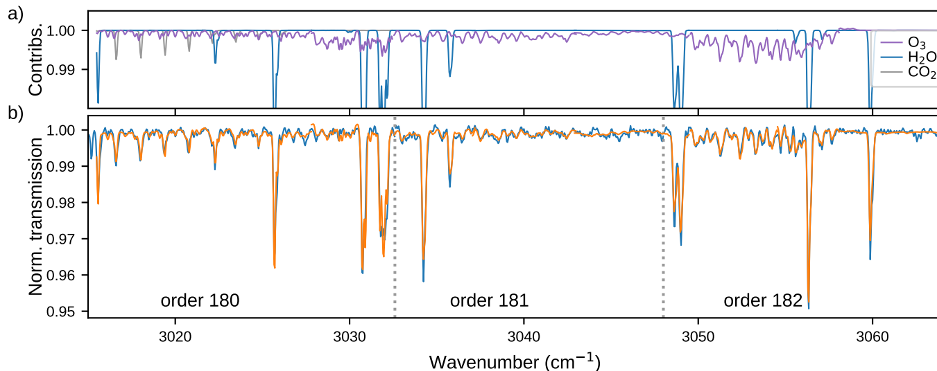
Fig. 1. Spectra recorded by ACS MIR at 5.5 km using secondary grating position 12 during occultation 2476 N1 on L_s = 192.7^\circ : (a) contributions from O_3 , H_2O , and CO_2 to the best-fit for orders 180–182; (b) data and best-fits for orders 180–182.
