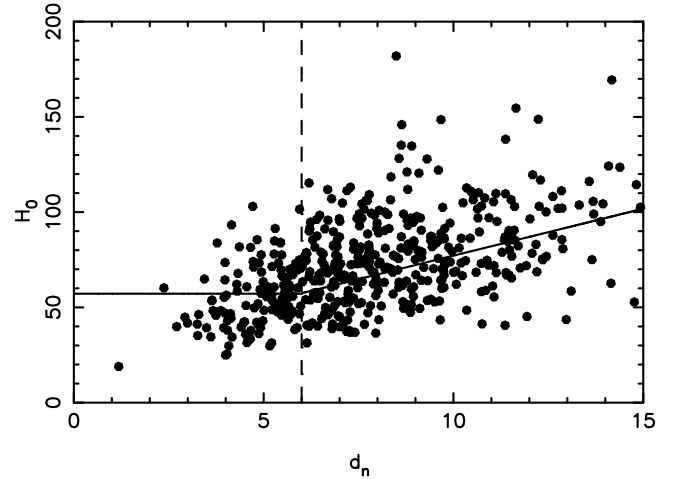
Fig. 6. Hubble constant versus the normalized distance for the basic sample. The curve represents the constant value of the Hubble parameter for the subsample when d_n \leq 6 and the increase of the parameter with a linear fit when d_n > 6 .
