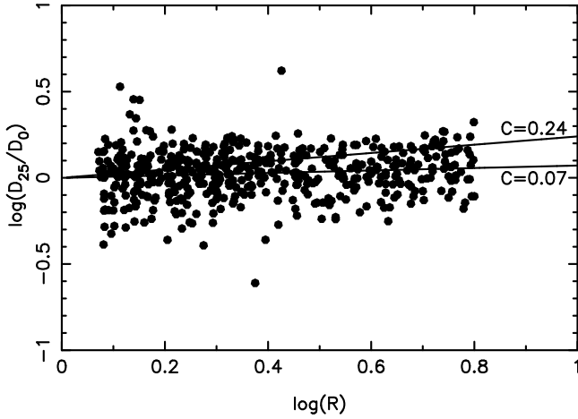
Fig. 10. \log(D_{25}/D_0) versus \log(R) for the basic sample. The upper line represents the result from the DL subsample with a slope C = 0.24 . The lower line is a fit for the data with a slope C = 0.07 .
