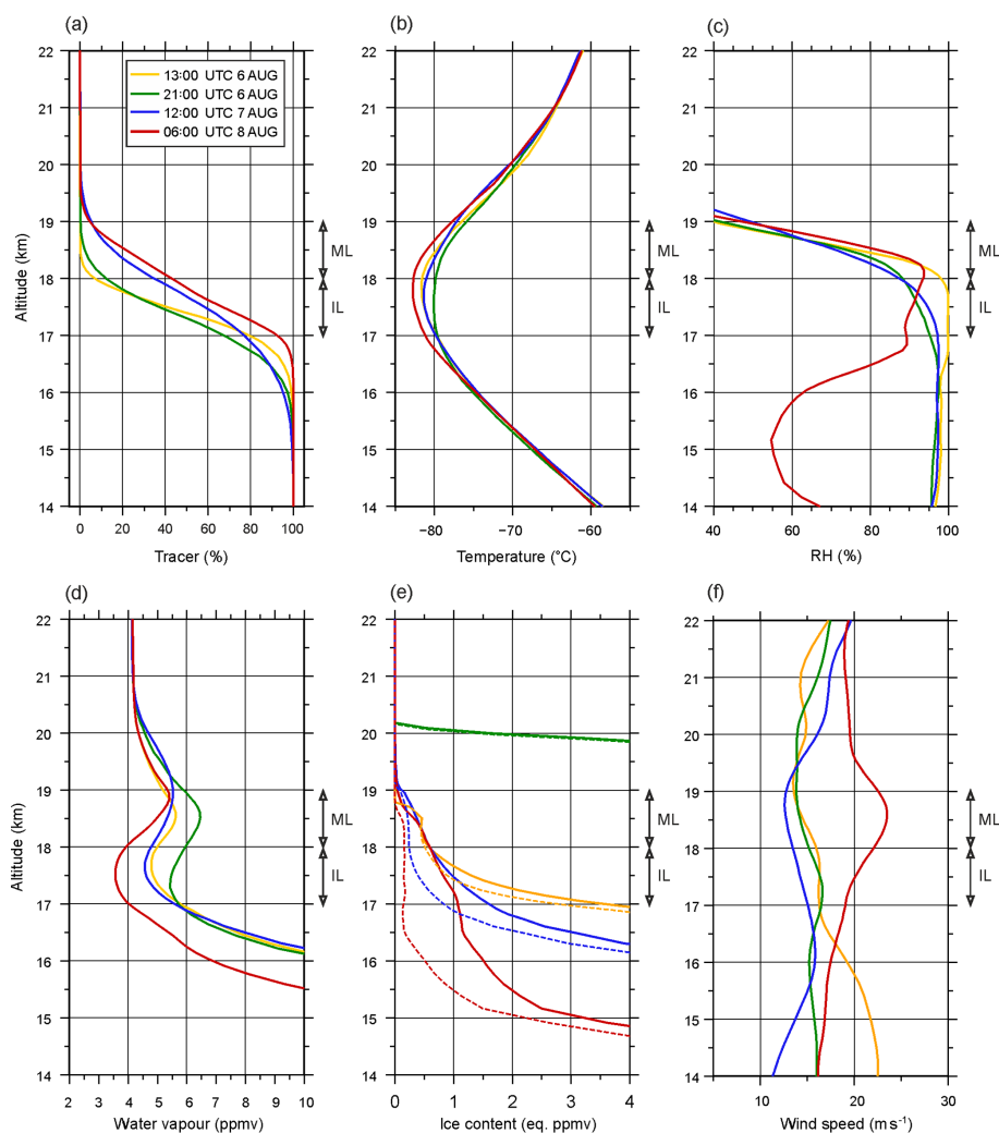
Figure 11. Vertical profiles of (a) tracer (%), (b) temperature ( ^{\circ}\text{C} ), (c) relative humidity (%), mixing ratios of (d) water vapour (ppmv), (e) ice content (eq. ppmv), and (f) wind speed ( \text{m s}^{-1} ) across the hydration patch along the trajectory at 13:00 UTC (yellow line), 21:00 UTC (green line) on 6 August, 12:00 UTC on 7 August (blue line), and 06:00 UTC (red line) on 8 August 2017. The layers of the ML and IL are marked by arrows. In (e), the ice content is depicted by solid lines, while the cloud ice is shown by dashed lines.
