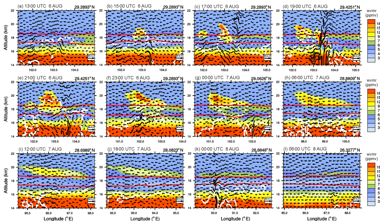
Figure 6. Vertical cross sections of water vapour mixing ratio (wvwr) (shading) and wind (vectors) at (a) 13:00 UTC, (b) 15:00 UTC, (c) 17:00 UTC, (d) 19:00 UTC, (e) 21:00 UTC, and (f) 23:00 UTC on 6 August 2017; (g) 00:00 UTC, (h) 06:00 UTC, (i) 12:00 UTC, and (j) 18:00 UTC on 7 August 2017; and (k) 00:00 UTC and (l) 06:00 UTC on 8 August 2017. The isentropic altitudes of 380 and 410 K are depicted by the red lines. The latitude ( ^{\circ} N) of west–east-oriented cross-section line is indicated at the upper right of each panel. The cloud boundary (mixing ratio of ice content of 10 \text{ mg kg}^{-1} ) is contoured by the white solid line.
