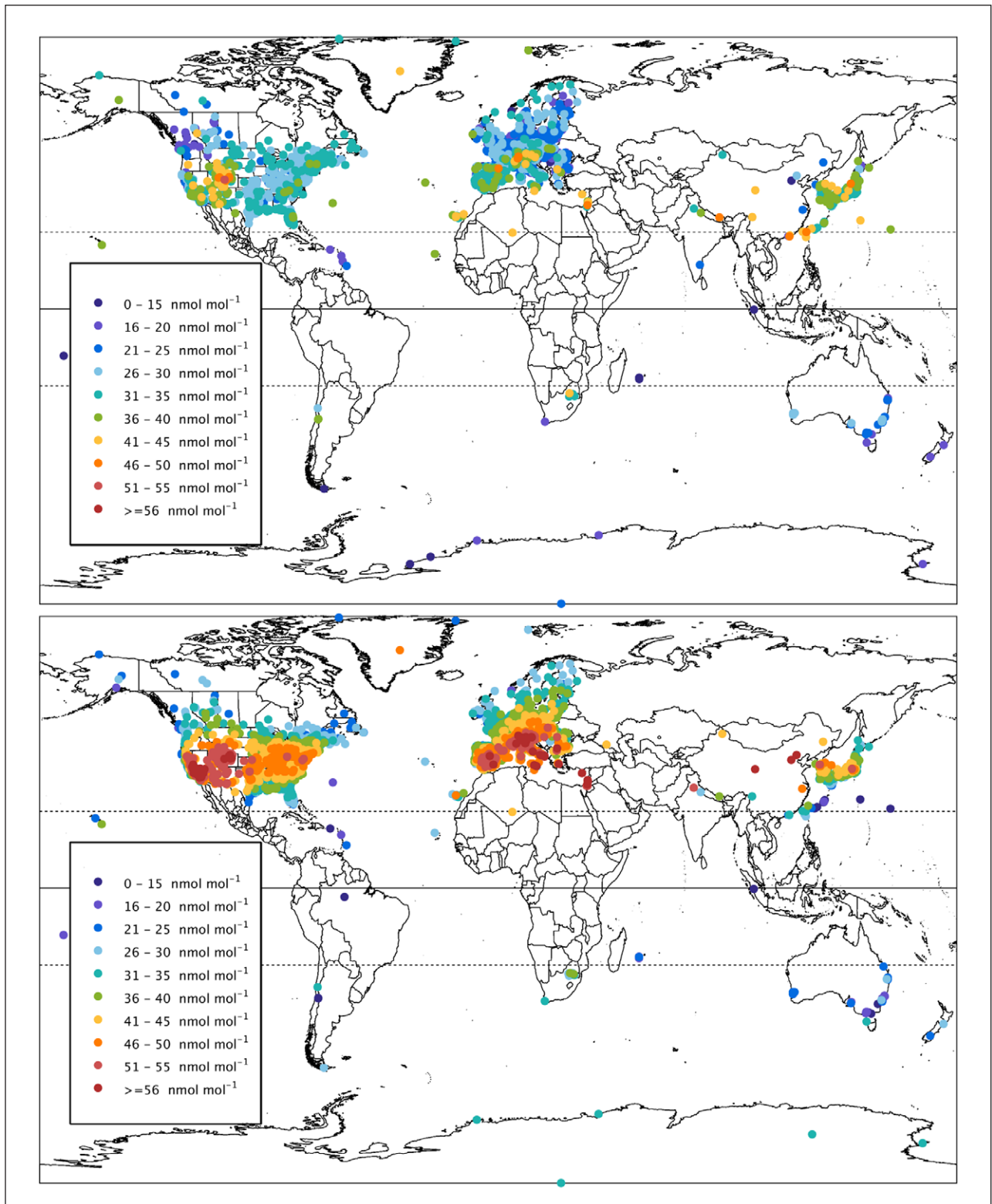
Figure 1: Present-day global daytime average ozone (nmol mol -1 ). Global daytime average ozone (nmol mol -1 ) at 2702 non-urban surface sites in December–January–February (top) and 3136 non-urban sites in June–July–August (bottom) for the present-day period, 2010–2014. DOI: https://doi.org/10.1525/elementa.291.f1
