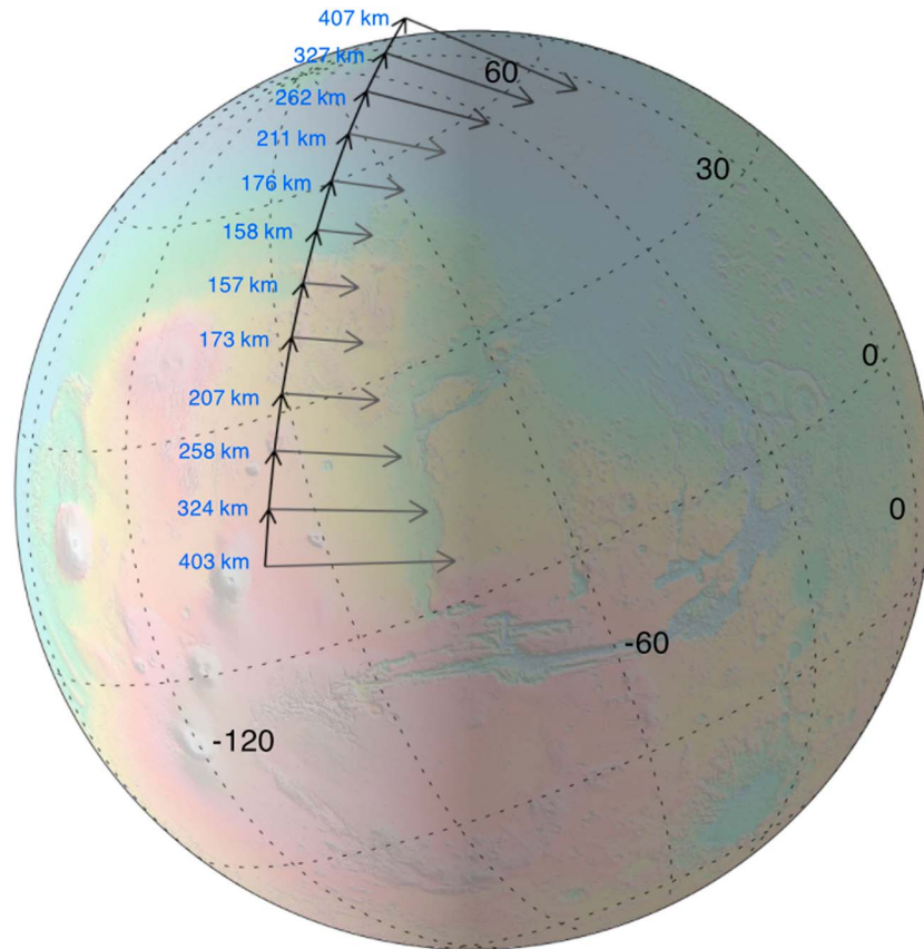
Figure 1. The MAVEN periape segment and IUVS observing geometry during flare orbit 5718 on 10 September, 17:35 UT. The tails of the vertical velocity vectors indicate the locations of the sub-spacecraft latitude and longitude during 12 IUVS limb scans. The numbers next to the velocity vectors indicate spacecraft altitude. The horizontal arrows show the latitude and longitude of the IUVS tangent lines of sight. The altitude of IUVS LOS roughly spans between 80 and 220 km. IUVS = Imaging Ultraviolet Spectrograph; LOS = line of sight.
