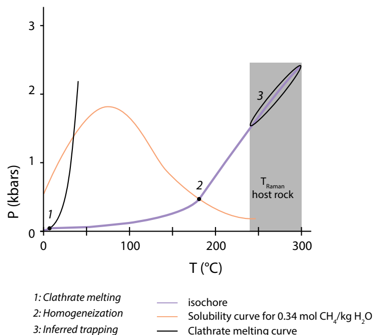
Figure 9. Representative isochore for the fluid inclusions from the Flysch à Helminthoïdes unit (FH), using values in Table 2 as to get an upper bound on trapping pressure. Trapping conditions are inferred at the intersection between the isochore and the temperature of host rock estimated with Raman (Table 1).
