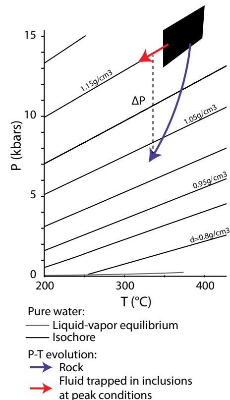
Figure 10. Concomitant evolution of rock (blue) and fluid inclusion (red) pressure-temperature (P-T) conditions during exhumation. The steeper slope of rock P-T path results in large overpressure \Delta P between the trapped fluid and the surrounding medium, eventually leading in the general case to reequilibrating the fluid. Rock peak conditions (black domain) and exhumation path from the Schistes Lustrés (SL) (Agard et al., 2000), fluid isochores calculated from Wagner and Pruss (2002) for pure water, with associated density. The isochore line passing through the peak P-T conditions corresponds to a T gradient of \sim 12 °C/km.
