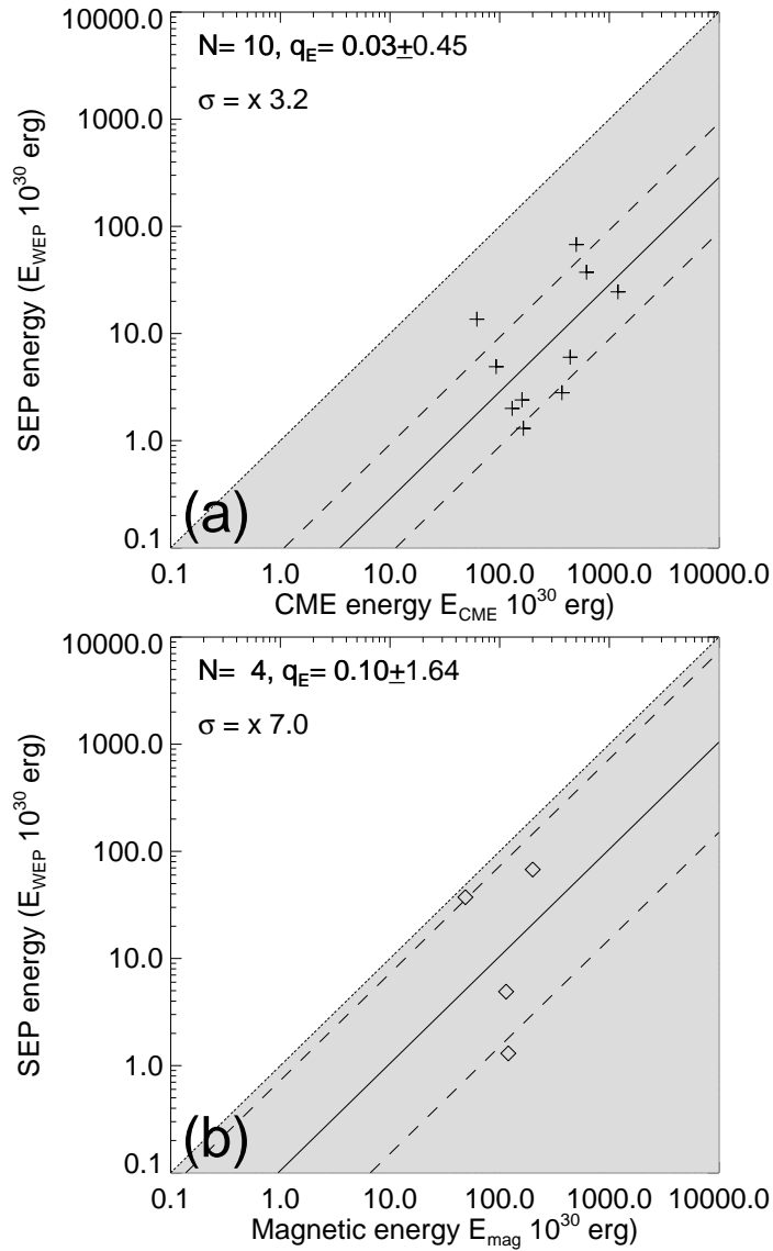
Fig. 9.— The ratio of SEP kinetic energies E_{SEP} to CME energies E_{CME} (a) and versus the dissipated magnetic energy E_{mag} in flares (b), based on the SEP data given in Table 1.
