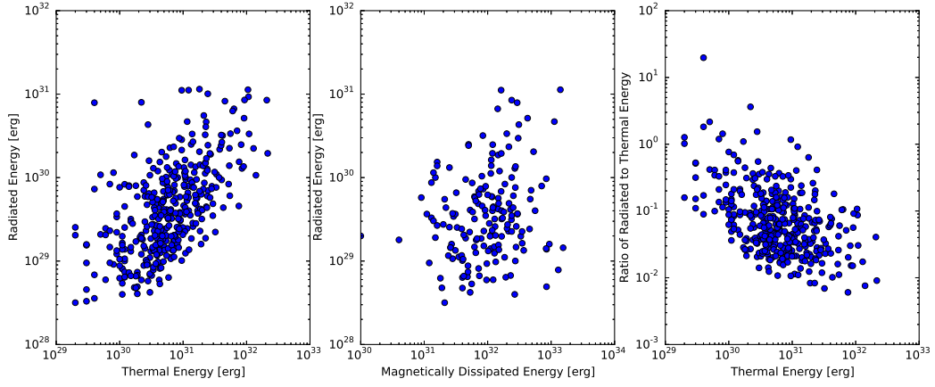
Fig. 7.— Thermally radiated energies from the hot ( >4 MK) coronal plasma as a function of thermal and magnetically dissipated energies: (a) Radiated energy versus thermal energy; (b) Radiated energy versus magnetically dissipated energies; and (c) Ratio of radiated to thermal energies versus thermal energy.
