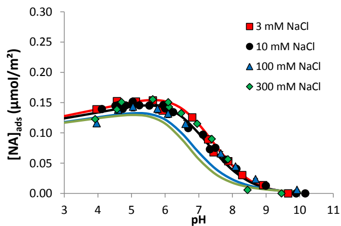
Figure S3. Modeling of single NA system, considering NA dimer formation at goethite surfaces (final model, see the main text for more details). Adsorption of 10 \mu\text{M} NA to goethite (0.5 g/L) versus pH and [NaCl] (3-300 mM). Solid lines are modeling results (the same color as the corresponding symbol).
