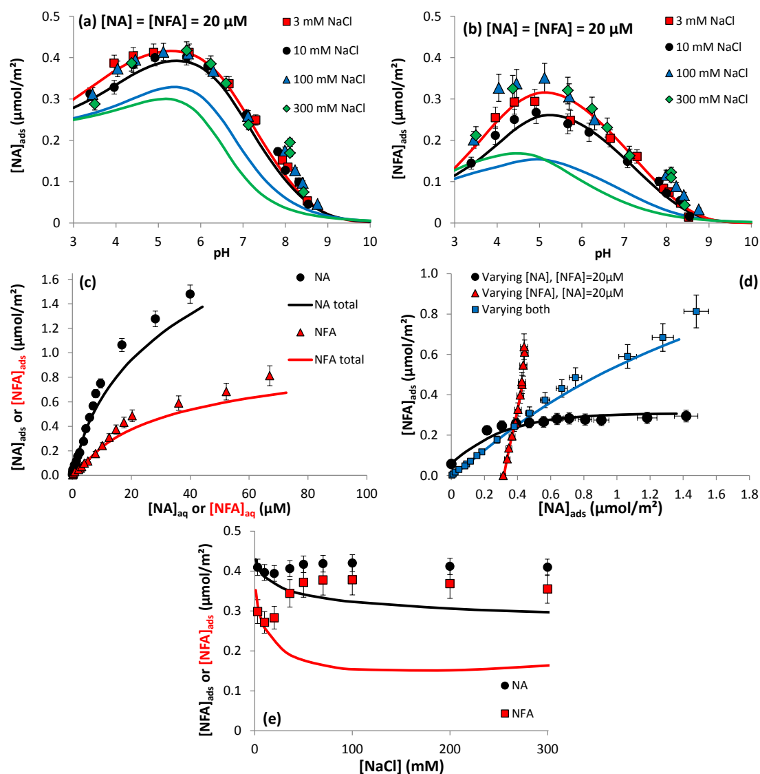
Figure S6. Experimental results and modeling data of binary NA-NFA system with NA-NFA dimer formation but without ion pair formation with sodium. Adsorption of (a) NA and (b) NFA to goethite (0.5 g/L) versus pH and [\text{NaCl}] (3-300 mM) for [\text{NA}]_{\text{tot}} = [\text{NFA}]_{\text{tot}} = 20 \mu\text{M} . (c) NA and NFA adsorption isotherms at pH 6 in 10 mM NaCl for [\text{NA}]_{\text{tot}} = [\text{NFA}]_{\text{tot}} . (d) [\text{NFA}]_{\text{ads}} vs [\text{NA}]_{\text{ads}} for three experimental conditions: (i) ( [\text{NFA}]_{\text{tot}} = 20 \mu\text{M} , varying [\text{NA}]_{\text{tot}} , black), (ii) ( [\text{NA}]_{\text{tot}} = 20 \mu\text{M} , varying [\text{NFA}]_{\text{tot}} , red), and (iii) varying both compounds with [\text{NA}]_{\text{tot}} = [\text{NFA}]_{\text{tot}} (blue). (e) Adsorption of NA and NFA ( [\text{NA}]_{\text{tot}} = [\text{NFA}]_{\text{tot}} = 20 \mu\text{M} ) on goethite (0.5 g/L) versus [\text{NaCl}] at pH 5. In all graphs, lines correspond to overall adsorption predicted by surface complexation modeling (using the same color as the corresponding symbol).
