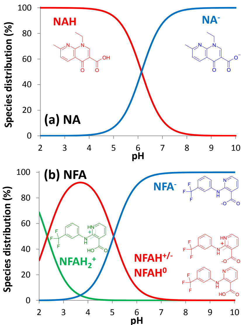
Figure S1. Distribution of (a) NA and (b) NFA at various pH values with molecular structures of different NA and NFA species. Ionic strength: 10 mM NaCl. pK_{a,s} of NA ( pK_a=6.19 ) and NFA ( pK_{a,1}=2.28 and pK_{a,2}=5.10 ) at infinite dilution were obtained from conditional pK_a values and the Davies equation.
