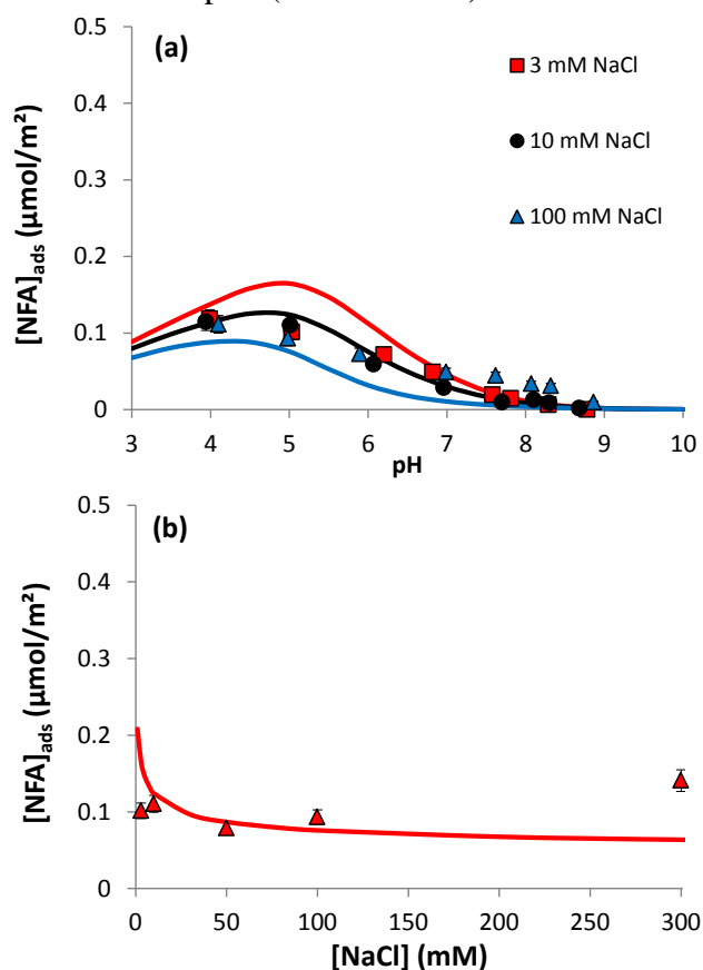
Figure S4. Modeling of single NFA system, without considering the formation of a sodium-NFA ion pair (preliminary model). (a) Adsorption of 20 μM NFA to goethite (0.5 g/L) versus pH and [NaCl] (3-100 mM). (b) Adsorption of 20 μM NFA to goethite (0.5 g/L) versus [NaCl] at pH 5. Solid lines are modeling results (the same color as the corresponding symbol).
