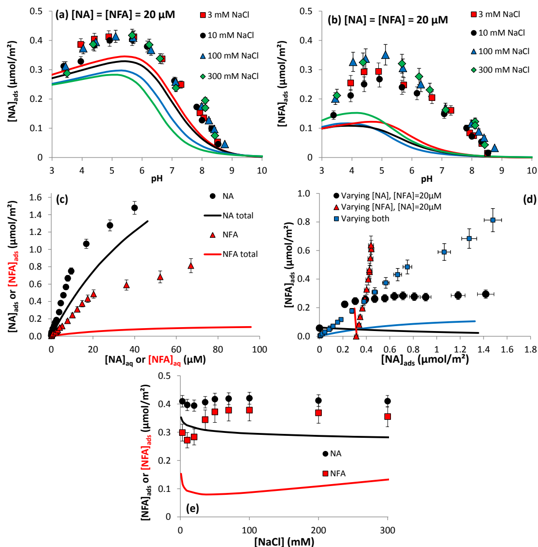
Figure S5. Experimental results and modeling data of binary NA-NFA system without NA-NFA dimer formation. Adsorption of (a) NA and (b) NFA to goethite (0.5 g/L) versus pH and [NaCl] (3-300 mM) for [NA]_{tot} = [NFA]_{tot} = 20 \mu\text{M} . (c) NA and NFA adsorption isotherms at pH 6 in 10 mM NaCl for [NA]_{tot} = [NFA]_{tot} . (d) [NFA]_{ads} vs [NA]_{ads} for three experimental conditions: (i) ( [NFA]_{tot} = 20 \mu\text{M} , varying [NA]_{tot} , black), (ii) ( [NA]_{tot} = 20 \mu\text{M} , varying [NFA]_{tot} , red), and (iii) varying both compounds with [NA]_{tot} = [NFA]_{tot} (blue). (e) Adsorption of NA and NFA ( [NA]_{tot} = [NFA]_{tot} = 20 \mu\text{M} ) on goethite (0.5 g/L) versus [NaCl] at pH 5. In all graphs, solid lines correspond to overall adsorption predicted by surface complexation modeling (using the same color as the corresponding symbol).
