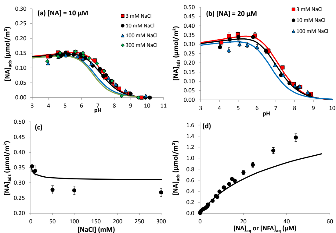
Figure S2. Modeling of single NA system, without considering NA dimer formation at goethite surface (preliminary model). (a) Adsorption of 10 μM NA to goethite (0.5 g/L) versus pH and [NaCl] (3-300 mM) (b) Adsorption of 20 μM NA to goethite (0.5 g/L) versus pH and [NaCl] (3-100 mM). (c) Adsorption of 20 μM NA to goethite (0.5 g/L) versus [NaCl] at pH 5. (d) NA-goethite adsorption isotherm at pH 6 in 10 mM NaCl.
