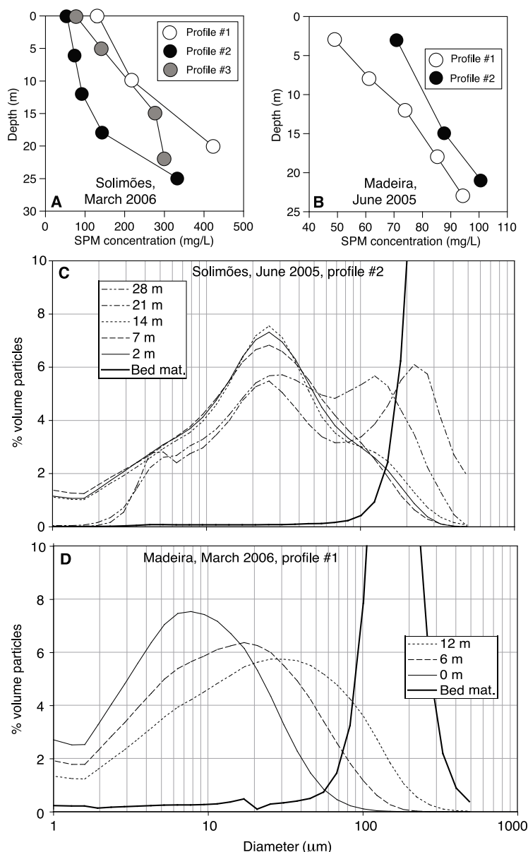
Figure 2. Representative suspended particulate matter (SPM) concentration depth profiles: (a) the Solimões River in March 2006, and (b) the Madeira River in June 2005. Representative grain size distributions in depth profiles: (c) the Solimões River in June 2005 and (d) the Madeira River in March 2006. See Table 1 for profiles and samples characteristics.
