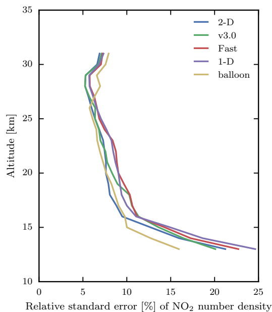
Figure 5. Relative standard error of coincident NO 2 profiles. Note that OSIRIS profiles have been scaled to various local times of the balloon measurements, which adds random error to the OSIRIS profiles due to random variations between the photochemical model atmosphere and the true atmosphere.
