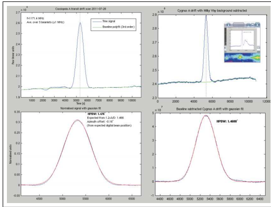
Figure 4. Cassiopeia-A and Cygnus-A observation
