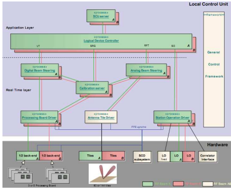
Figure 2. Control architecture
