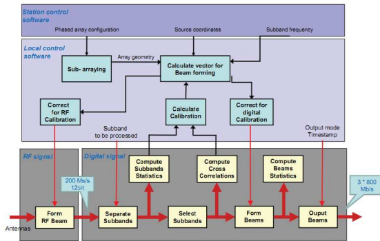
Figure 1. RF and Digital EMBRACE Processing
