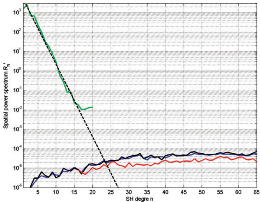
Figure 3. Mauersberger–Loves spectra of the lithospheric contributions to the temporal changes of the field of internal origin at the Earth’s mean radius, as predicted from the VIS grid of Hemant & Maus (2005), using xCHAOS up to degree 16 at epoch 2004, as input for the time-varying inducing field (black); the same VIS grid but using the average secular variation (between 1960 and 2002.5) up to degree 13 of CM4 (blue), using MF5 divided by 1000 yr (red). Also shown the spectrum of xCHAOS secular variation for epoch 2004 (green) and a best linear fit to this spectrum up to degree 16 (dashed, R'_n = 10^{-0.3728n+4.0654} ). Units are (\text{nT yr}^{-1})^2 .
