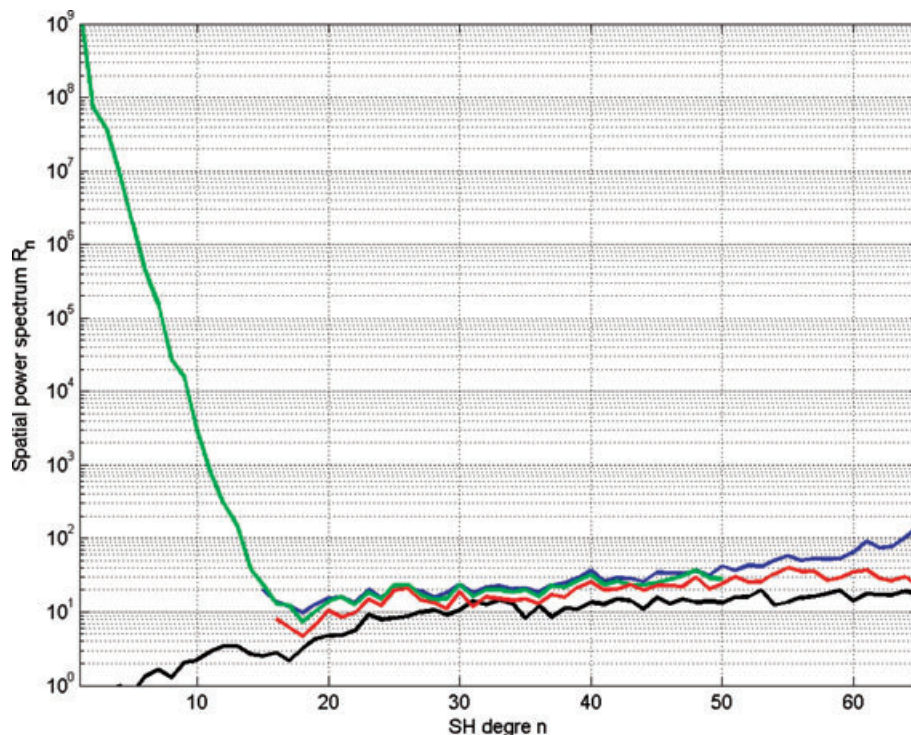
Figure 2. Mauersberger–Loves spectrum of the induced lithospheric field predicted at the Earth’s mean radius by the VIS grid of Hemant & Maus (2005) when using xCHAOS (up to degree 13, for epoch 2004), as the inducing field (black). For comparison, the Mauersberger–Loves spectra of the field of internal origin at the Earth’s mean radius as estimated from the CM4 model of Sabaka et al. (2004) (blue), the MF5 model of Maus et al. (2007) (red), the xCHAOS model of Olsen & Mandaia (2008) (green) are also shown. Note that MF5 is only a model of the lithospheric field for degrees 16–100. Units are (nT) 2 .
