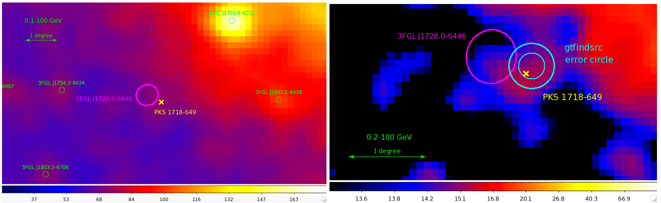
FIG. 1.— Left: Fermi -LAT 0.1-100 GeV count map of the sky centered on the radio position of PKS 1718–649 (yellow cross). The pixel size is 0.2 degrees/pixel. The magenta ellipse gives the uncertainty position (95% confidence level) of 3FGL J1728.0–6446 reported in the 3FGL. Field \gamma -ray sources in the 3FGL are indicated with green circles. Right: Zoom on the PKS 1718–649 region at >200 MeV energies. The pixel size is 0.1 degrees/pixel. The cyan circles correspond to the gtfindsrc best fit position (68% and 95% confidence levels).
