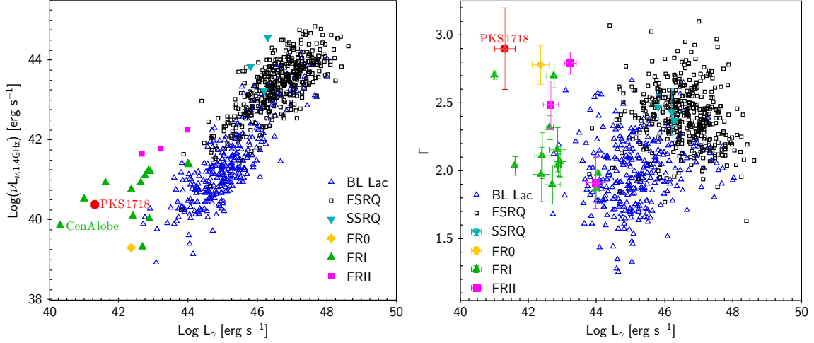
FIG. 2.— Left: Radio luminosity of the 3LAC FR I (solid, green triangles) and FR II (solid, magenta squares) radio galaxies, BL Lacs (open, open triangles), FSRQs (open, black squares), and SSRQs (cyan, solid triangles) plotted as a function of the \gamma -ray luminosity between 1 GeV and 100 GeV. We included Tol1326-379 (solid, yellow diamond), classified as FR 0 (Grandi et al. 2015), and the \gamma -ray detected lobes of Centaurus A (the south lobe with measured \gamma -ray and 1.4 GHz fluxes, see Abdo et al. 2010b and Hardcastle et al. 2009, respectively). The position of PKS 1718–649 is indicated by the solid, red circle. Right: \gamma -ray spectral index versus 1-100 GeV luminosity. PKS 1718–649 is located in the MAGN region of the diagram, with values of \Gamma and L_{\gamma} similar to those of Centaurus A. (Sample data: courtesy of P. Grandi.)
