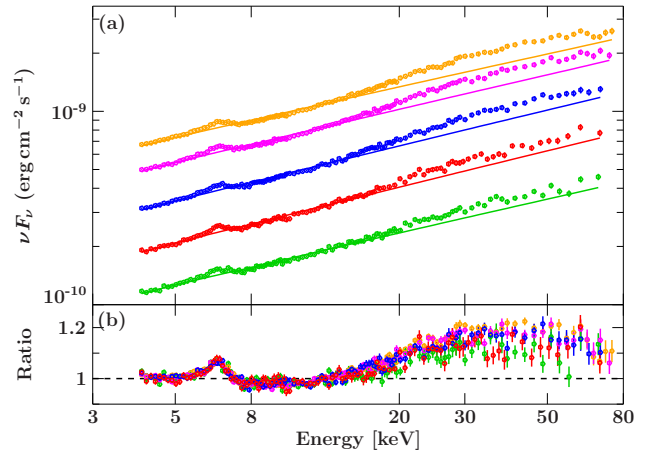
FIG. 3.— (a) Unfolded spectra of all five observations. Only NuSTAR /FPMA data are shown for clarity. Observation I is shown in red, observation II in blue, observation III in magenta, observation IV in orange and observation V in green. (b) Ratio residuals to a simple power-law fit. See text for details.
