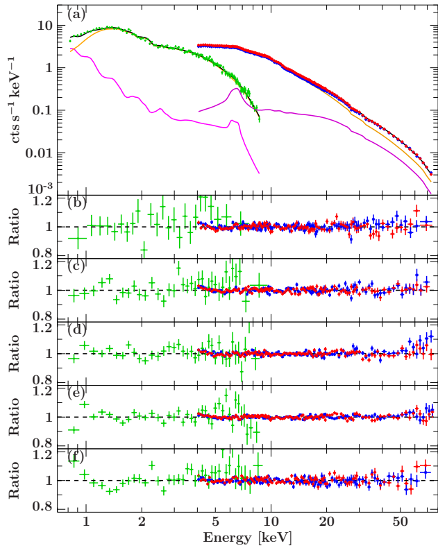
FIG. 5.— (a) Data and best-fit model for M2-q3 for observation IV, showing the reflection component in magenta and the power-law components in orange. Swift /XRT data are shown in green, NuSTAR /FPMA in red, and FPMB in blue. (b)–(f) Residuals in terms of model to data ratio of the best-fit model for observation I–V, respectively. Data were rebinned for clarity. See Table 2 for the model parameters.
