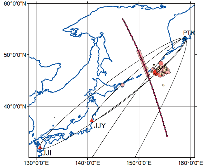
Figure 1. Map showing the positions of the Petropavlovsk-Kamchatsky (PTK) station and the JJI and JJY VLF/LF transmitters, together with the epicenters of the earthquake on November 15, 2006, and its aftershocks (after the US Geological Survey catalog). The ellipses show the sensitivity zones for the JJI, JJY and NWC transmitters. Part of a night-time orbit of the DEMETER satellite that passes above the earthquake area is indicated. Pink rectangle, section where effects are observed.
