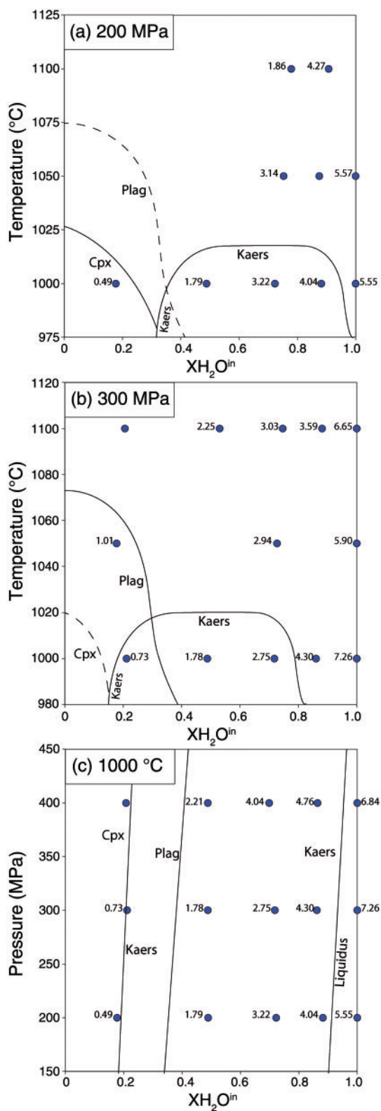
Fig. 4. Isothermal (a, b) and isobaric (c) phase diagrams illustrating the stability fields of different phases in AW experiments. Numbers next to points indicate wt % H 2 O dissolved in the glass of the experimental charge as measured by FTIR spectroscopy. Although not shown, titanomagnetite is ubiquitous in all charges. Apatite was not always detected but is inferred to be stable in runs below ~1100°C. A dashed line indicates an inferred phase boundary.
