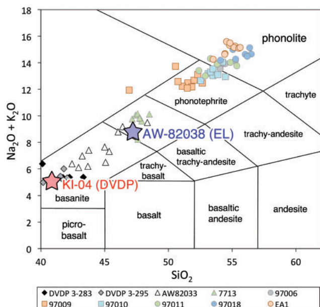
Fig. 3. Total alkalis vs silica (TAS) diagram showing the compositions of the starting materials (stars) relative to the fractional crystallization sequence seen in Erebus Lineage rocks represented by a suite of melt inclusions [data from Oppenheimer et al. (2011)].
