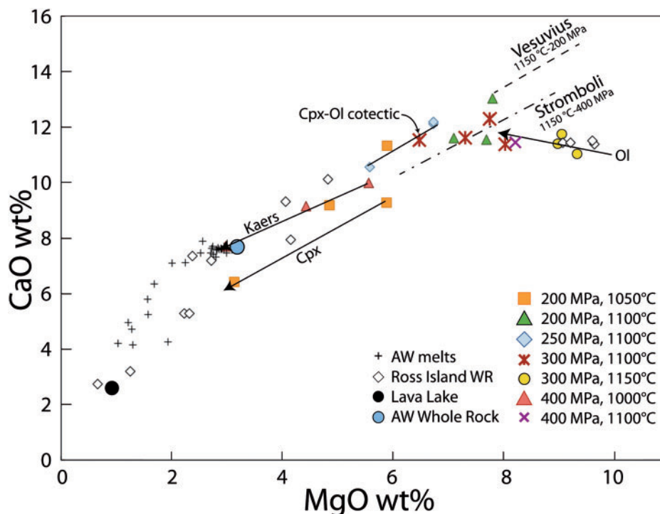
Fig. 9. CaO vs MgO plot showing the compositions of cotectic and near-cotectic experimental glasses, which mimic natural whole-rock compositions from a suite of Ross Island lavas (open diamonds), useful in identifying trends in compositions dominated by the precipitation of olivine and Ca-pyroxene (or amphibole). KI runs are shown with different symbols in terms of P - T conditions. The Cpx- Ol cotectic at 1050°C is shown for KI melts. Also plotted are experimentally determined Cpx- Ol cotectics for melts from Stromboli (Pichavant et al. , 2009) and Vesuvius (Pichavant et al. , 2014). Despite compositional differences in the starting materials used in these three studies, mafic alkali-rich liquids saturated in Cpx \pm Ol and kaersutite define a relatively narrow evolutionary trend in this diagram. KI melts are marked by initial Ol crystallization, followed by either Cpx \pm Pl or Kaers.
