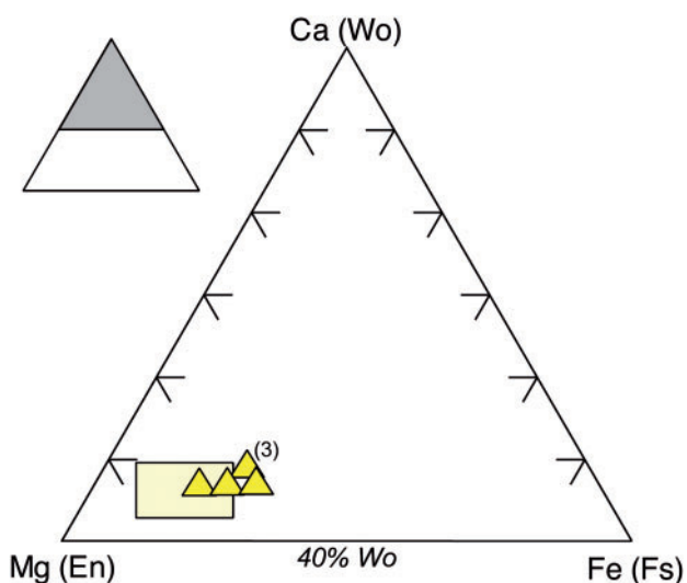
Fig. 10. Enlarged ternary diagram (from 40% Wo) showing the compositions of experimental (symbols) and natural (yellow box) clinopyroxenes, plotted in terms of recalculated end-member compositions enstatite, ferrosilite and wollastonite. The number (3) indicates three samples with the same composition.
