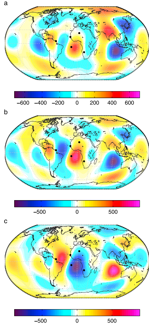
Figure 3. Maps of (a) \Delta\ddot{B}_r at epoch 2003, (b) \ddot{B}_r at epoch 2005 and (c) \Delta\ddot{B}_r at epoch 2007 at the core surface from the CHAOS-2 model. Black dots indicate the positions of observatories listed in Table 1. Unit: nT/yr 2 .
