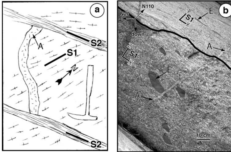
Figure 2. Late Variscan high-temperature foliation in the Mont Blanc granite. (a) Sketch of an aplitic dike (A) crosscutting the Mont Blanc granite “magmatic” foliation S1. S1 and the dike are crosscut by two alpine shear zones (S2). Eperon des géographes above the Leshaux glacier. Horizontal plane, view from above. Hammer gives scale. (b) Undeformed aplitic dike cutting across a flattened (S1) enclave of the Mont Blanc granite. North bank of the Leshaux glacier under the Talèfre glacier. View toward the east of two perpendicular planes: N20 vertical and N110 30S.
