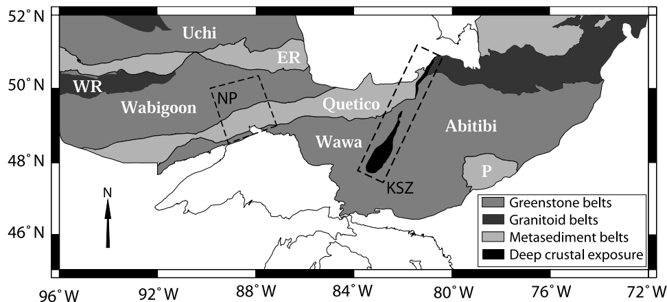
Figure 2. Generalized geological map of the Superior Province of the Canadian Shield showing major subprovinces from Card and Ciesielski [1986] and J. Percival (personal communication, 2005). ER is the English River metasedimentary subprovince, WR is the Winnipeg River plutonic subprovince, and P is the Pontiac metasedimentary subprovince. The boxes show the location of the Nipigon Embayment (NP) and the Kapuskasing Structural Zone (KSZ).
