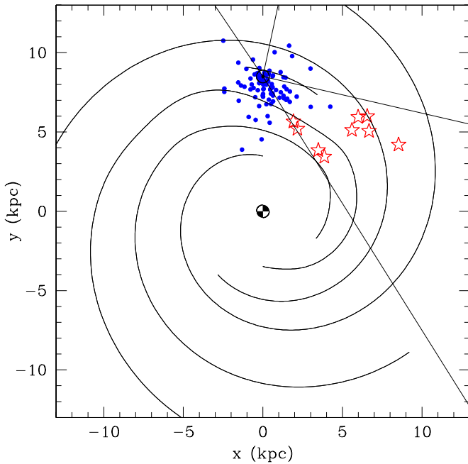
Figure 7. Overhead Galactic projection plot showing the nominal locations of 90 known field radio MSPs in the ATNF catalog with P < 25 ms and \dot{P} < 10^{-17} (blue dots) and 9 known PALFA MSPs (red stars) (Champion et al. 2008; Knispel et al. 2010, 2011; Deneva et al. 2012), including the 4 described in this paper. The nominal distances are inferred from the DMs and are uncertain by \sim 30\% . The Sun is located at the center of the cluster of dots, and the Galactic center is at the origin. The black curves indicate locations of the Galactic spiral arms according to the NE2001 model of Cordes & Lazio (2002). The cones indicated by the two pairs of straight lines indicate the regions of the Galactic plane that are visible from Arecibo. The PALFA MSPs are among the most distant non-cluster MSPs known.
