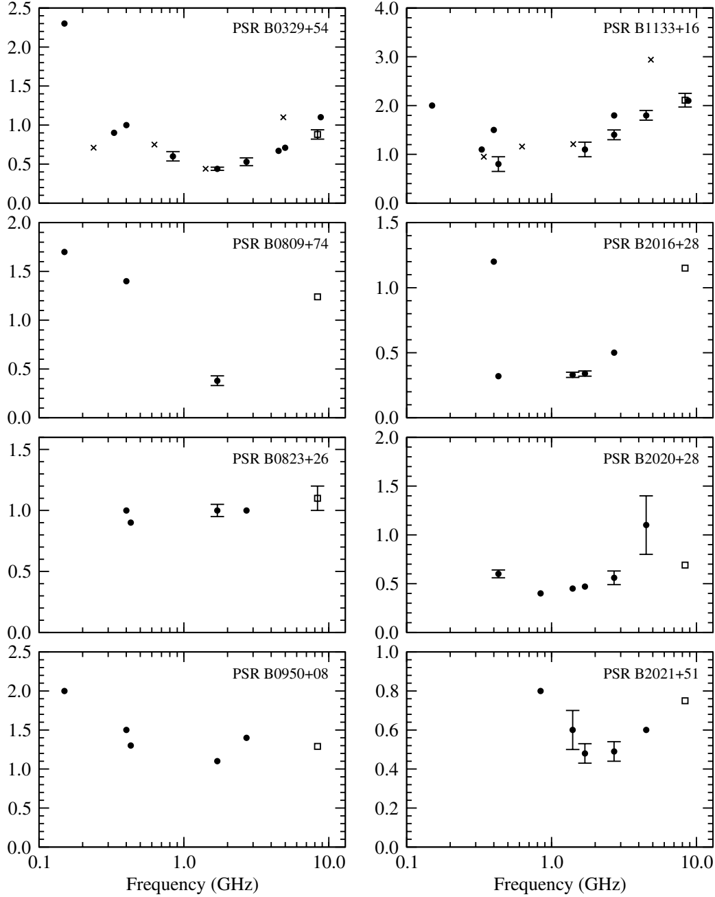
Fig. 4. Modulation indices m versus frequency for the observed pulsars. It is clearly seen that m_{\text{int}} first decreases with frequency, and after it reaches so-called critical frequency \nu_m^c (which for all, except B0823+26, is around 1 GHz), it rises again. Filled circles and crosses denote values taken from Bartel et al. (1980) and Kramer et al. (2003), respectively. Open squares represent values obtained in this work.
