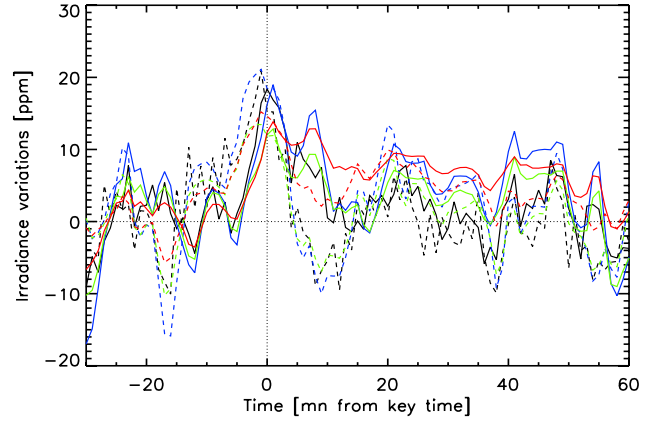
Fig. 2. Influence of the key time on the analysis. Dashed lines are average flare time series using the GOES 0.1–0.8 nm flux peak time, thick lines are average flare time series using the peak time of the derivative of the GOES 0.1–0.8 nm flux. Black is for TSI, red for 862 nm, blue for 402 nm, and green for 500 nm. The average is made over the 150 largest flares in our sample, from X28 to M5.
