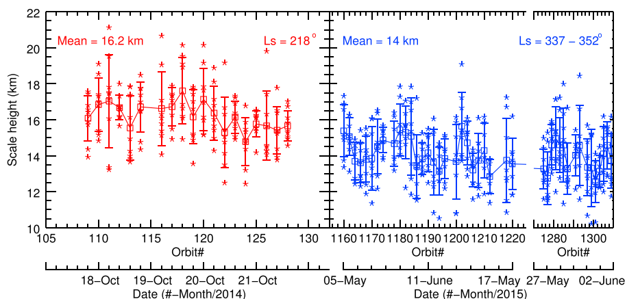
Figure 4. Variation of \text{CO}_2^+ ultraviolet doublet scale height for two seasons. Symbol shows the derived scale height for each individual scan in an orbit. Thick colored lines show the mean scale height and thin lines show the standard deviation for each orbit. The mean scale height for L_S = 218^\circ and L_S \sim 345^\circ are 16.2 \pm 0.12 km and 14 \pm 0.1 km, respectively. The error on scale height determination is smaller than the observed variations within an orbit.
