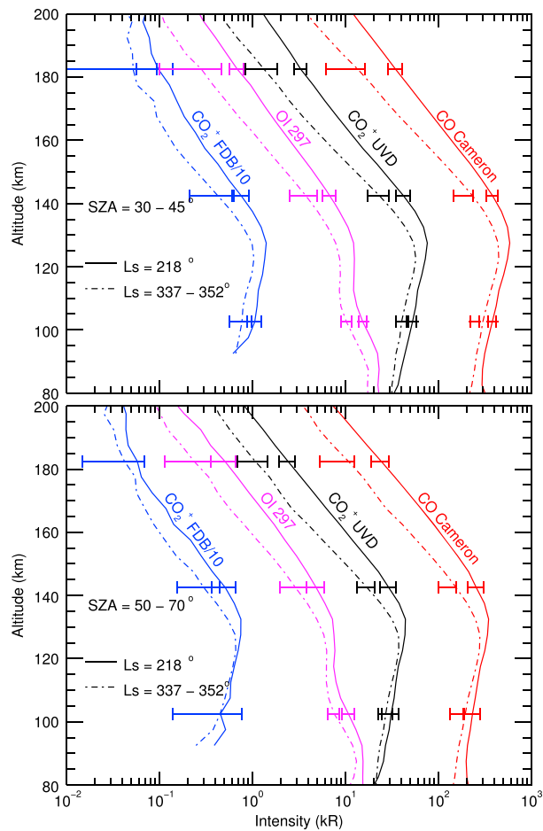
Figure 2. Mean altitude profiles for the \text{CO}_2^+ ultraviolet doublet, CO Cameron band, OI 297.2 nm, and \text{CO}_2^+ Fox-Duffendack-Barker bands for two solar longitudes and (top) SZA = 30–45° and (bottom) SZA = 50–70°. Solid curves show the brightness for L_S = 218^\circ , and dash-dotted curves shows them for L_S \sim 345^\circ . The intensity of \text{CO}_2^+ FDB band is divided by a factor of 10. Horizontal bars show the standard deviation of the profiles. The intensities decrease by ~50% for SZA = 50–70°.
