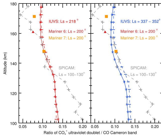
Figure 3. Ratio of Cameron band and \text{CO}_2^+ UVD for (left) L_S = 218^\circ and (right) L_S \sim 345^\circ seasons and \text{SZA} = 30\text{--}45^\circ (solid curves) and 50\text{--}70^\circ (dashed curve). Gray dashed curves: intensity ratio taken for SPICAM measurements carried out at L_S = 100\text{--}130^\circ and \text{SZA} = 15\text{--}37^\circ [Leblanc et al. , 2006]. Triangle: intensity ratio deduced by Leblanc et al. [2006] for Mariner 6 at \text{SZA} = 27^\circ and L_S = 200^\circ . Squares: intensity ratio deduced by Leblanc et al. [2006] for Mariner 7 at \text{SZA} = 44^\circ and L_S = 200^\circ .
