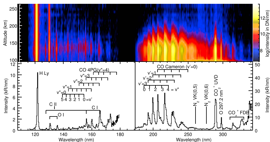
Figure 1. (top) The IUVS's FUV and MUV detectors color composite generated using a full vertical scan from orbit 110 (2059 UTC, 18 October 2014), one of the 744 profiles. The horizontal and vertical axes represent wavelength and altitude (80–250 km), respectively. (bottom) Calibrated FUV and MUV spectra obtained from the same scan; these are averages of 13 individual spectra obtained between 120 and 135 km.
