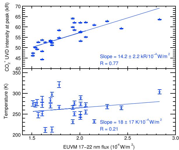
Figure 5. Short-term variations of (top) \text{CO}_2^+ doublet maximum intensity and (bottom) topside temperature with 17–22 nm irradiance measured by the EUVM instrument aboard MAVEN. Values are for L_S \sim 337\text{--}343^\circ (orbits 1160–1220) and SZA between 30^\circ and 40^\circ . R is the linear correlation coefficient.
