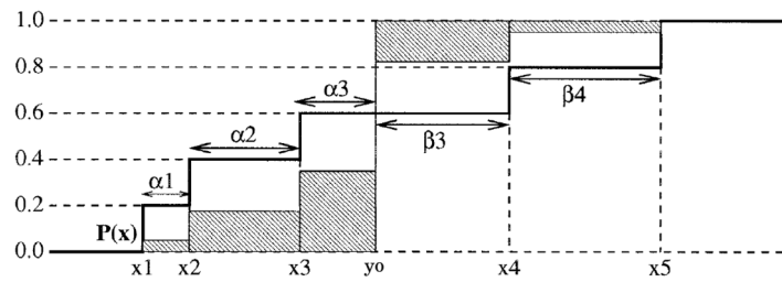
Figure 18. Illustration of the CRPS computation (according to Hersbach [2000]). The cumulative distribution for an ensemble of five members ( x_1, \dots, x_5 ) and the verifying observation y_o is shown. The CRPS is represented by the shaded area.
