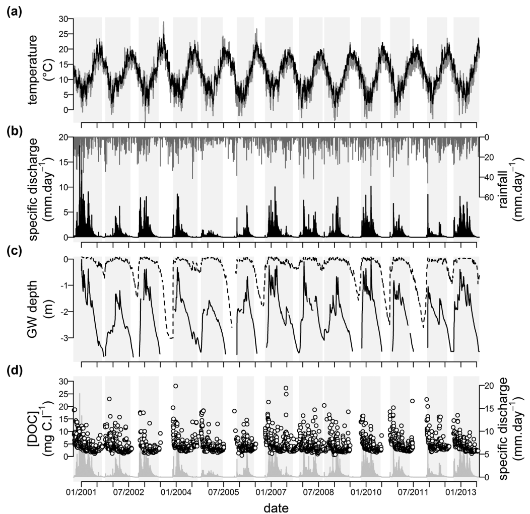
Figure 3. Variations in seasons, temperature, rainfall, discharge, groundwater table (GW) depth, and dissolved organic carbon (DOC) concentrations over the study period. Wet and dry seasons are superimposed onto each plot in gray and white, respectively. Due to an absence of GW measurements, no dry season is identified before 1 January 2001. (a) Air and soil ( -0.1 m) temperatures (gray and black lines, respectively). (b) Daily rainfall (gray lines) and daily discharge (black line). (c) Groundwater dynamics in wetland (dashed line) and upland soils (solid line). (d) Daily DOC concentrations (unfilled black circles) and daily discharge (gray line).
