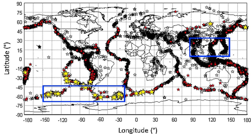
Figure 3. Distribution of all EQs with good detection corresponding to different number of perturbations. The white, red, and yellow stars are related to EQs with 1–9 perturbations, 10–19 perturbations, and more than 19 perturbations, respectively. Zone1 and Zone2 are indicated with blue rectangles (see text for explanation).
