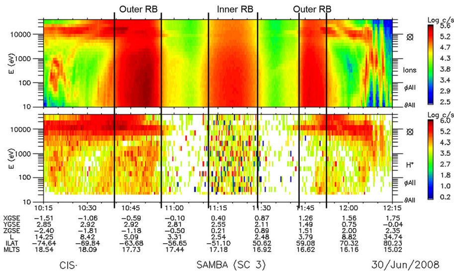
Figure 7. Energy-time spectrograms of ions (in counts/s) observed by CIS onboard C3 on 30 June 2008, between 10:15 and 12:15 UT, at about 16:00–18:00 MLT: HIA ions (top panel) and CODIF H^+ (bottom panel). The locations of the radiation belt boundaries as identified from the detected background are indicated by black vertical lines. Orbital parameters are indicated at the bottom of the figure. (Adapted from Ganushkina et al. [2011]).
