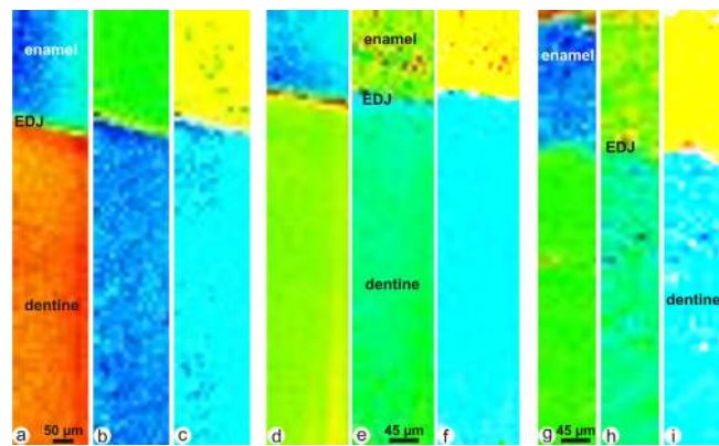
Fig. 6. FTIR maps of area between 900 and 1200 cm -1 for the mineral content (PO 4 ) (a, d, g), between 1580 and 1720 cm -1 for organic content (b, e, h). These maps are ratioed to estimate the mineral–organic ratios (c, f, i). a–c: Rattus , d–f: fresh Meriones , g–i: pellet from Bubo . The organic contents of both fresh and pellet Meriones differ from that of Rattus .
