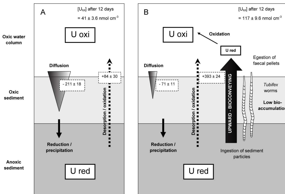
Figure 7. Conceptual outline of the repartition and transfers of U within a sediment without macro-invertebrate (A) or bioturbated by T. tubifex worms (B) under an oxygenated water column (U oxi = U in oxidized form, U red = U in reduced form). Framed values indicate the estimated fluxes of U over the 12 days of experiment ( 10^{-3} nmol cm -3 h -1 ): diffusion values correspond to diffusive fluxes estimated with PROFILE software; outward flux values, i.e. desorption/oxidation ± removal by bioturbation, correspond to variation of U concentration in water column in [U-12] and [UT-12] aquaria, respectively.
