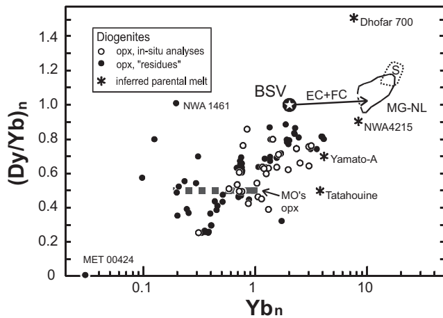
Fig. 2. (\text{Dy}/\text{Yb})_n ratios versus \text{Yb}_n for eucrites—MG-NL: main group and Nuevo Laredo trend eucrites, S: Stannern trend eucrites, data from Shimizu and Masuda (1986), Barrat et al. (2000, 2007) and orthopyroxenes from diogenites (in situ analyses from Fowler et al. [1995] and Beck et al. [2013], residues after leaching from Barrat et al. [2010]). The data are normalized to CI chondrites. The trend produced by equilibrium crystallization (EC) and fractional crystallization (FC) of a melt with a starting composition equivalent to the bulk silicate Vesta (BSV) is shown for comparison. Selected partition coefficients for low-Ca pyroxene ( D_{\text{Yb}} = 0.1 and D_{\text{Dy}}/D_{\text{Yb}} = 0.5 ) are used to calculate the compositions of the orthopyroxenes in equilibrium with the melts from the crystallizing magma ocean and from replenished shallow magma chambers (MO's opx). The same partition coefficients are used to estimate the parental melts of some diogenites—Tatahouine, Yamato-74013, NWA 4215, Dhofar 700. The pyroxenes from the diogenites and olivine (or harzburgitic) diogenites display the same range of \text{Dy}/\text{Yb} ratios, and have not been distinguished here.
