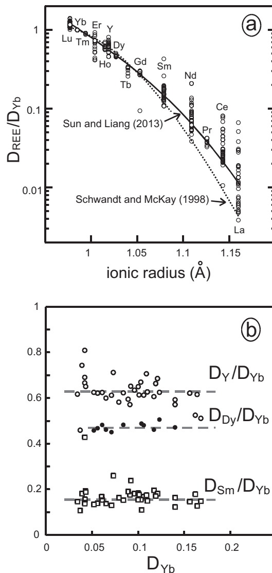
Fig. 1. Onuma diagram for ratios of experimental partition coefficients of trivalent REEs and Y for low-Ca pyroxenes (a), and selected ratios of partition coefficients for the same experiments (b). Data are from Blinova and Herd (2009), Frei et al. (2009), McDade et al. (2003a, 2003b), Salters and Longhi (1999), Salters et al. (2002), Schwandt and McKay (1998), Sun and Liang (2013), Van Kan Parker et al. (2010, 2011), and Yao et al. (2012). The scatter shown by the ratios of partition coefficients reflects, at least partly, the precision of the experimental data, which have not been filtered here. Notice that the spread of the experimental data is more limited for the heavy REE than for the light REE. Measured D_{\text{Dy}}/D_{\text{Yb}} ratios close to 0.5 are consistent with parameterized lattice strain models—e.g., Schwandt and McKay (1998) and Sun and Liang (2013).
