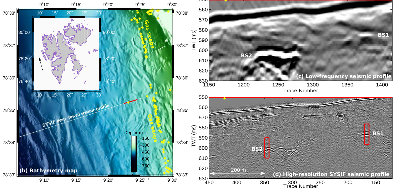
Figure 1. (a) Geographical location, shown by the black arrow and (b) bathymetric map of the study area, offshore Svalbard, in which there are numerous gas seeps (Westbrook et al. 2009). (c) Low-frequency seismic profile, shown in (a) by the red line, acquired in 2008 with an air-gun seismic source (30–150 Hz). Two bright-spot reflections located by the red boxes (BS1 and BS2) have been interpreted as gas-charged layers. (d) High-frequency seismic profile at the same location acquired in 2011 with the SYSIF deep-towed seismic device (220–1050 Hz).
