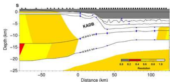
Figure 9. Resolution parameter for depth nodes of the velocity model. The depth uncertainties of the most important boundaries calculated from the 95% confidence limit of the f -test are given in the framed boxes (Figure 10). Velocity nodes are indicated by blue circles.
