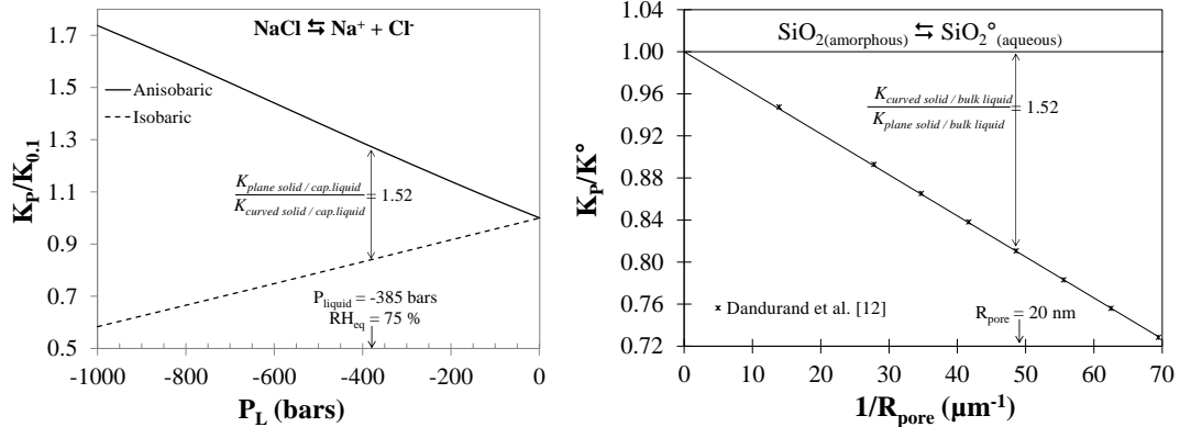
Fig. 2. Isobaric and anisobaric contexts illustrated for (a) NaCl solubility as a function of liquid pressure; (b) amorphous silica solubility as a function of pore radius (compared to experiments from [12]).
