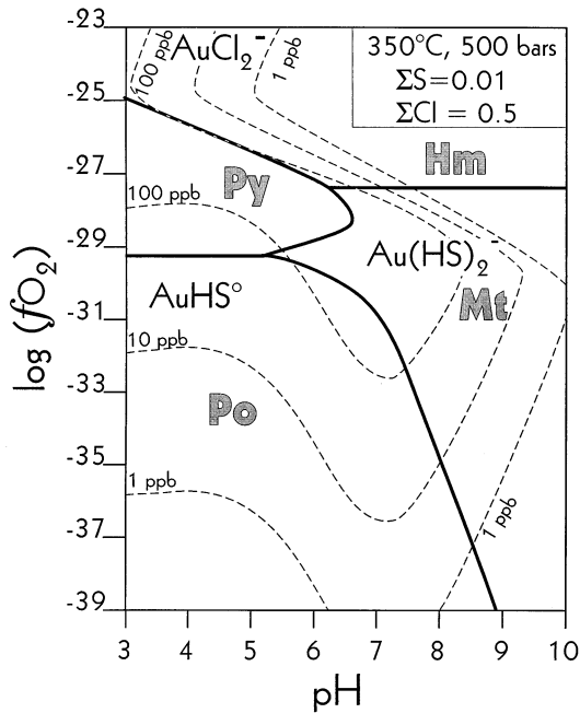
Fig. 14. Solubility contours for gold ( \Sigma\text{Au} = m\text{AuCl}_2^- + m\text{AuHS}^\circ + m\text{Au}(\text{HS})_2^- ) in a solution of T=350^\circ\text{C} , 500 bar, \Sigma\text{S} = 0.01 , and \Sigma\text{Cl} = 0.5 , shown as a function of f\text{O}_2 and pH.
