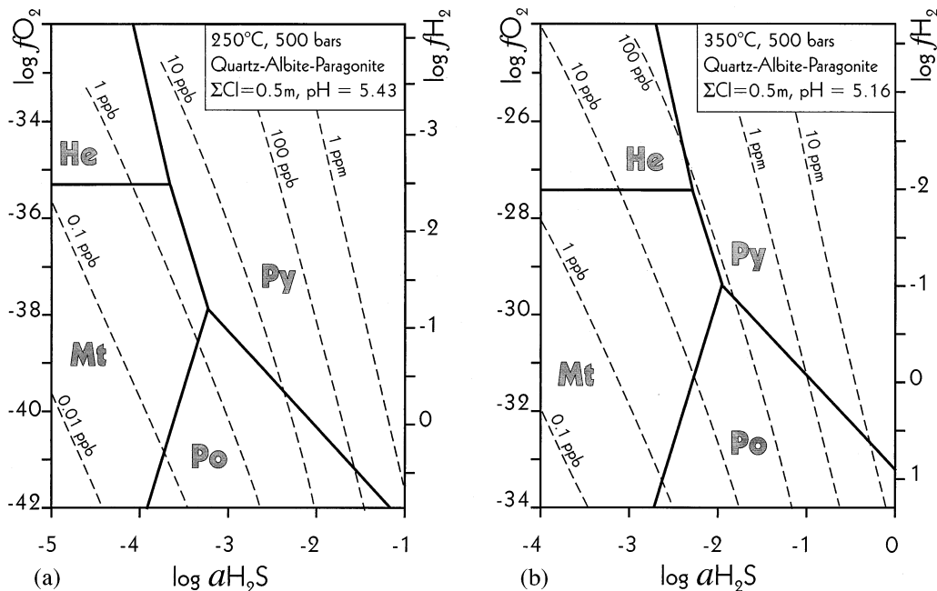
Fig. 15. Calculated solubility of gold at 250^\circ\text{C} (a) and 350^\circ\text{C} (b), computed as a function of f\text{O}_2 and a\text{H}_2\text{S}(\text{aq}) for a 0.5\text{ m NaCl} aqueous solution in equilibrium with the quartz-albite-paragonite pH buffer. The dashed lines represent the solubility contours of gold ( \Sigma\text{Au} = m\text{AuCl}_2^- + m\text{AuHS}^\circ + m\text{Au}(\text{HS})_2^- ). The solid lines separate the stability fields of pyrite, pyrrhotite, magnetite, and hematite.
