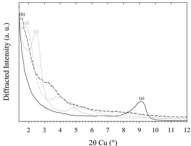
Fig. 2 : XRD patterns for (a) Na-Mt in black line, (b) Na-Mt with lysozyme in black dash line, (c) C_{10}E_3 -Mt synthesized by using C_{10}E_3 surfactant in gray line and (d) C_{10}E_3 -Mt with lysozyme in gray dash line. Large peaks for the layered materials without lysozyme (a), (c) and with lysozyme (b), (d) correspond to d_{001} reflections at 1.2 or 3.6 nm, and at 5.4 and 4.6 nm.
