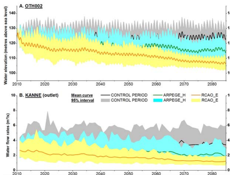
Figure 12. (a) Mean groundwater levels (30 scenarios) and 95% interval at observation point OTH002, (b) mean annual water flow rates (30 scenarios) and 95% interval at Kanne, for the control simulations and the climate models ARPEGE_H and RCAO_E.
