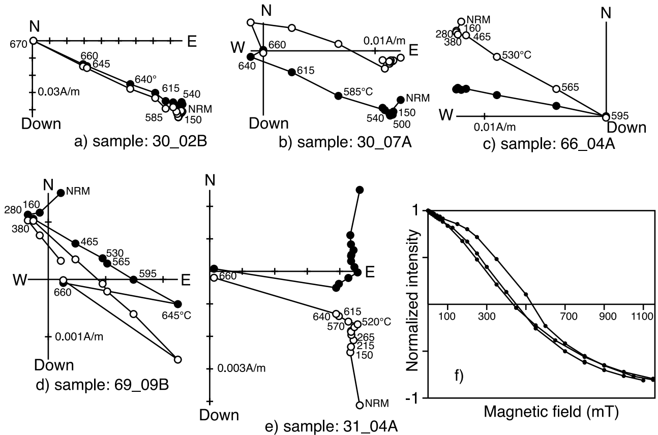
Figure 7. (a–e) Orthogonal plots of thermal demagnetization of samples from Paleogene red beds of the Chahuanca area. Open circles are projection in the vertical plane, while circles correspond to the horizontal plane. (f) Back field IRM acquisition after saturation in a field of 2.5 T for red bed samples.
