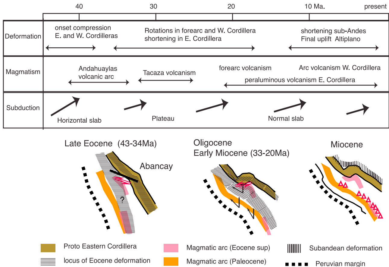
Figure 15. Summary of the geodynamic evolution of the southern Peruvian Andes since the middle Eocene. The Abancay line limits domains of central and southern Peru with different paleogeographic evolution [Carlotto et al. , 2009] and the protodeflection was enhanced during Tertiary Andean deformation. A flat slab episode was proposed by James and Sacks [1999].
