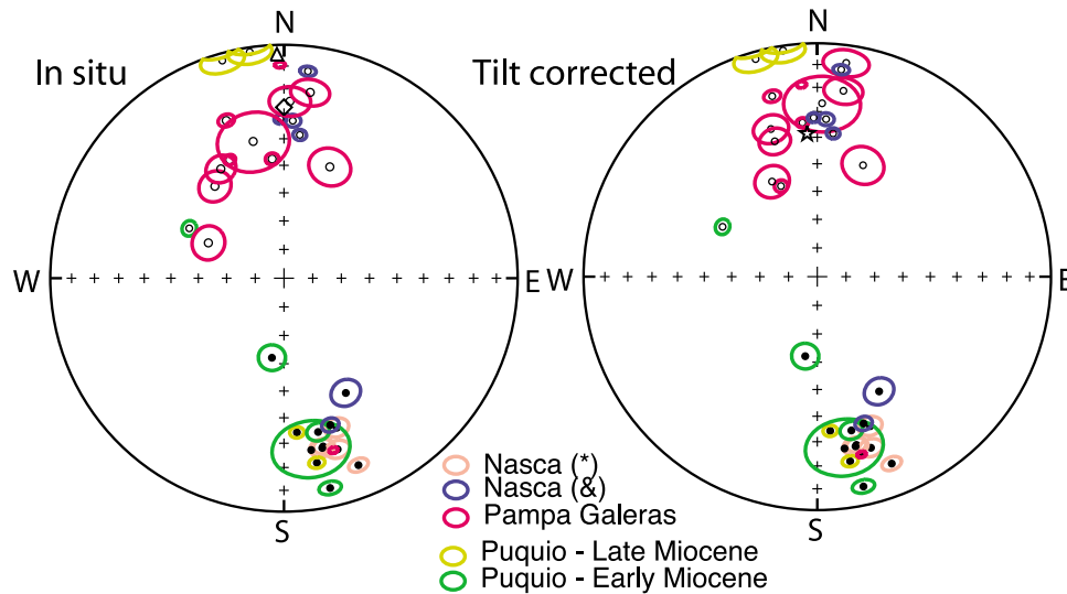
Figure 6. Equal-area stereonet of ChRM directions ((left) in in situ coordinate and (right) tilt-corrected coordinate) and 95% confidence angle around the mean for sites in the Puquio area. Open (solid) circles are projections in the upper (lower) hemisphere. The color of the confidence ellipse is used to separate the different data sets. Results in the Nazca ignimbrites are from Macedo-Sánchez et al. [1992b] (asterisk) and this study (ampersand). The triangle, diamond, and star are the present-day field direction, the geocentric axial dipole direction, and the expected direction at 20 Ma, respectively, from the Besse and Courtillot [2002] APWP for the South American plate.
