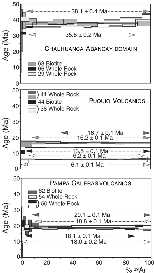
Figure 5. The ^{40}\text{Ar}/^{39}\text{Ar} data for sites in the Pampa Galeras, the Puquio area, and the Chalhuanca area.
