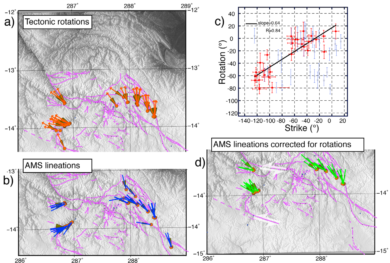
Figure 13. Summary of paleomagnetic results in the Chalhuanca-Cuzco area including results shown by Roperch et al. [2010]. (a) Tectonic rotations determined from the ChRM directions. (b) AMS lineations. (c) Oroclinal test with tectonic rotations versus strike of bedding (gray circles) or versus AMS lineations (red circles); (d) AMS lineations unrotated using the tectonic rotations calculated for each site.
