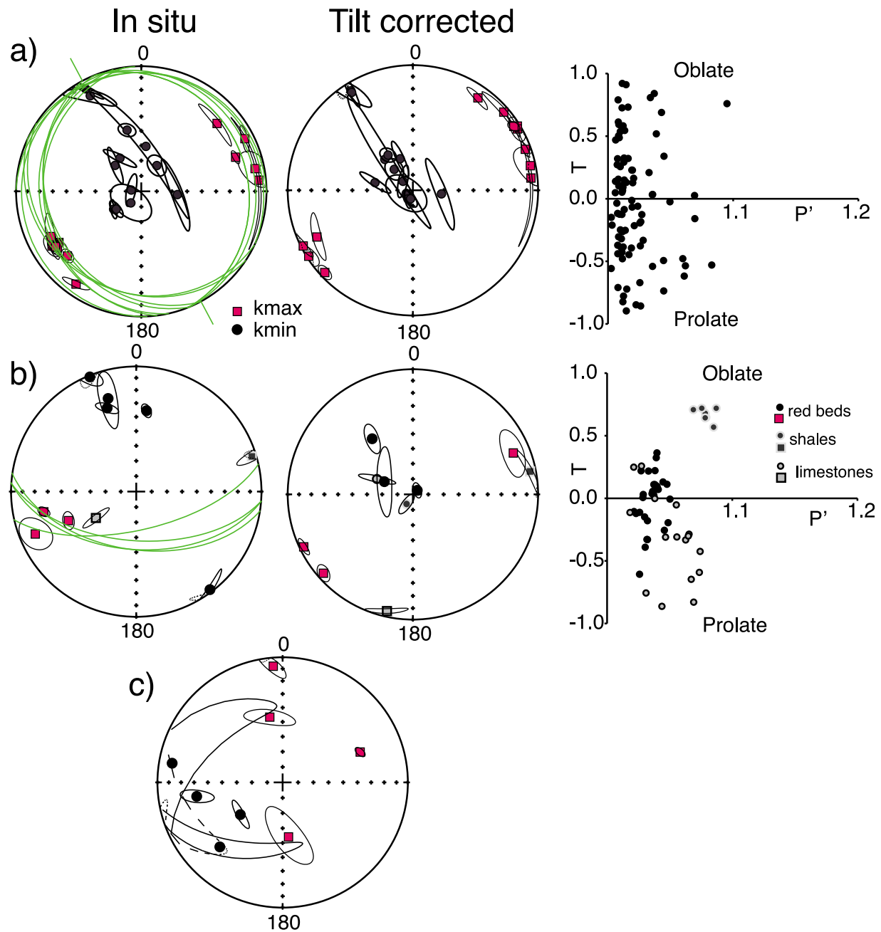
Figure 12. Equal-area projections of AMS results in (left) in situ and (middle) after bedding correction and (right) T-P' plot showing the shape of the AMS ellipsoids. (a) Red beds of the Chalhuanca area. (b) Copacabana limestone and black shales at site 75 and red beds of the Andahuaylas area. (c) AMS results in intrusive stocks of the Chalhuanca-Andahuaylas area. In Figures 12a and 12b, great circles in green correspond to bedding. In Figure 12a the orientation of the syncline determined from the bedding measurements is also highlighted by two short line segments.
