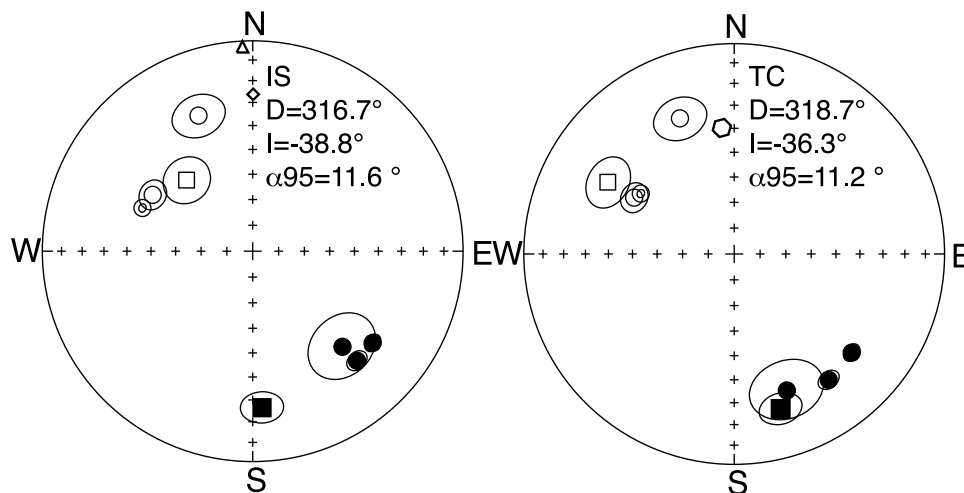
Figure 11. Paleomagnetic results for the Anta domain shown in (left) in situ and (right) tilt-corrected coordinates. The squares correspond to results from site 3 with the low unblocking temperatures of reverse polarity and the high unblocking temperature component with normal polarity. Circles correspond to volcanic rocks. The secondary component of reverse polarity at site 3 is not used to calculate the mean. The triangle, diamond, and hexagon are the present-day field direction, the geocentric axial dipole direction, and the expected direction at 40 Ma, respectively.
