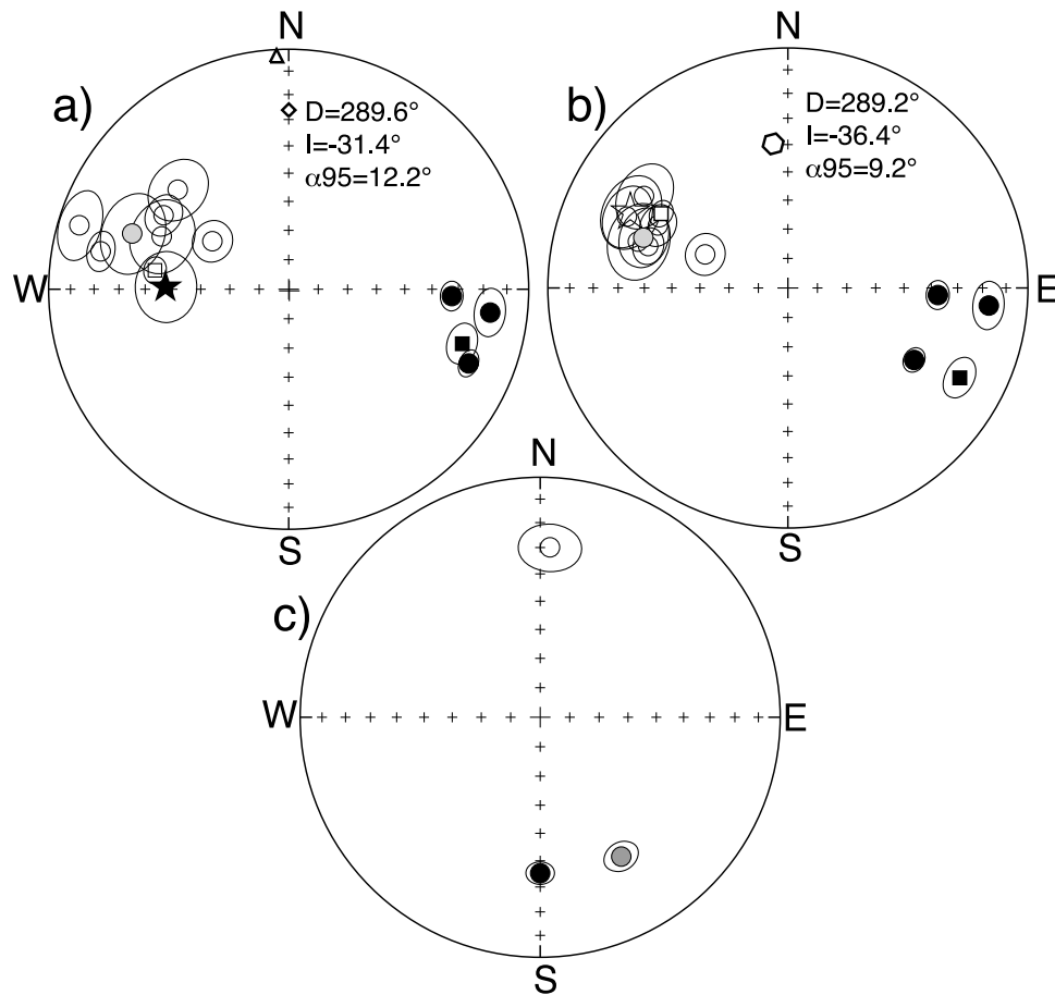
Figure 9. Equal-area stereonets of ChRM directions in (a) in situ and (b) after bedding correction for sites north of Chalhuanca. Circles are results in red beds and baked contacts, squares correspond to the antipodal magnetizations in limestones at site 72, and the star corresponds to the nonremagnetized limestone at site 71. The triangle, diamond, and hexagon are the present-day field direction, the geocentric axial dipole direction, and the expected direction at 40 Ma, respectively, from the Besse and Courtillot [2002] APWP for the South American plate. (c) Results in intrusive stocks 27 and 73 and remagnetized Jurassic black shales at site 34 (gray square).
