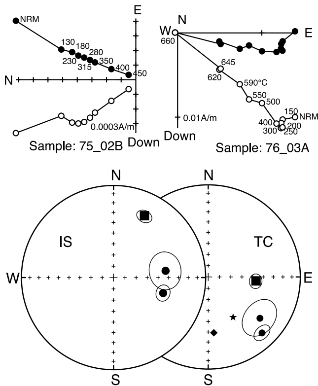
Figure 10. (top) Orthogonal plots of thermal demagnetization for one sample from site 75 and one sample from site 76. (bottom) Equal-area stereonets of ChRM directions in lower Permian black shales (site 75, square) and Paleogene red beds (sites 76 and 77, circles). The diamond and star are the expected direction at 40 Ma and 290 Ma, respectively, for the stable South American plate.
