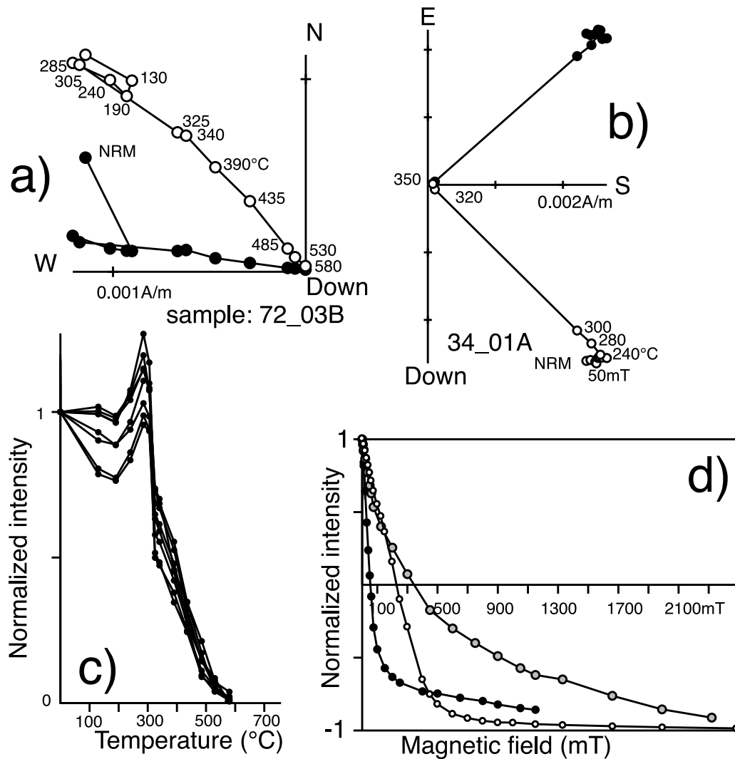
Figure 8. (a) Orthogonal plot of thermal demagnetization of one sample in remagnetized limestones at site 72. A normal polarity is observed above 285°C. A component of magnetization of opposite polarity is observed in the temperature range 150°C–285°C. (b) Orthogonal demagnetization of one sample from the Jurassic black shales at site 34. The sample was first submitted to AF demagnetization up to 50 mT and thermally demagnetized from 190°C up to 350°C. The ChRM, likely carried by pyrrhotite, is unblocked between 300°C and 320°C. (c) Variation in the intensity of the magnetization after demagnetization in zero field for all samples of site 72 in the Ferrobamba limestone. (d) Back field IRM acquisition after saturation in a field of 2.5 T. The gray circles correspond to one sample from site 72. The white circles correspond to one sample in remagnetized black shales from site 34. The solid circles correspond to one sample in nonremagnetized Ferrobamba limestone at site 71.
