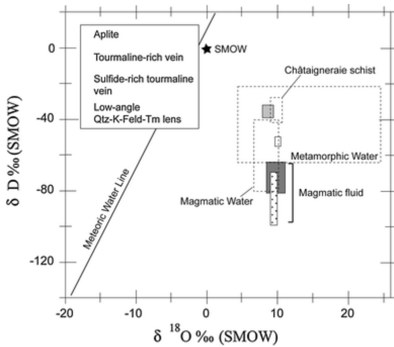
Fig. 11 Report of the analyzed tourmaline within a \delta^{18}\text{O} vs \delta\text{D} diagram in order to compare and discuss their formation with respect of the theoretical magmatic and metamorphic fields. Domain of tourmaline in micaschist found within the La Chataigneraie district is indicated for discussion (Lerouge et al. 2000). Qtz quartz, K-feld potassic feldspar, Tm tourmaline
