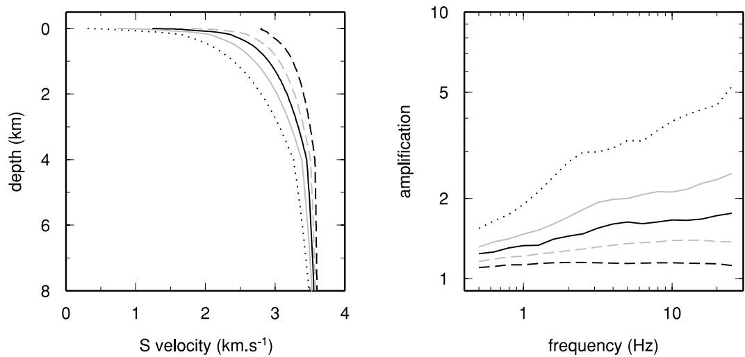
Figure 2. Left-hand side: generic rock velocity profiles (e.g. Boore & Joyner 1997; Cotton et al. 2006) with different v_{s30} values: 500 \text{m s}^{-1} (black dotted line), 1000 \text{m s}^{-1} (grey line), 1500 \text{m s}^{-1} (black line), 2000 \text{m s}^{-1} (grey dashed line) and 3000 \text{m s}^{-1} (black dashed line). Right-hand side: generic amplifications resulting from the profiles on the left for vertically incident SH waves, using a Haskell–Thomson procedure.
