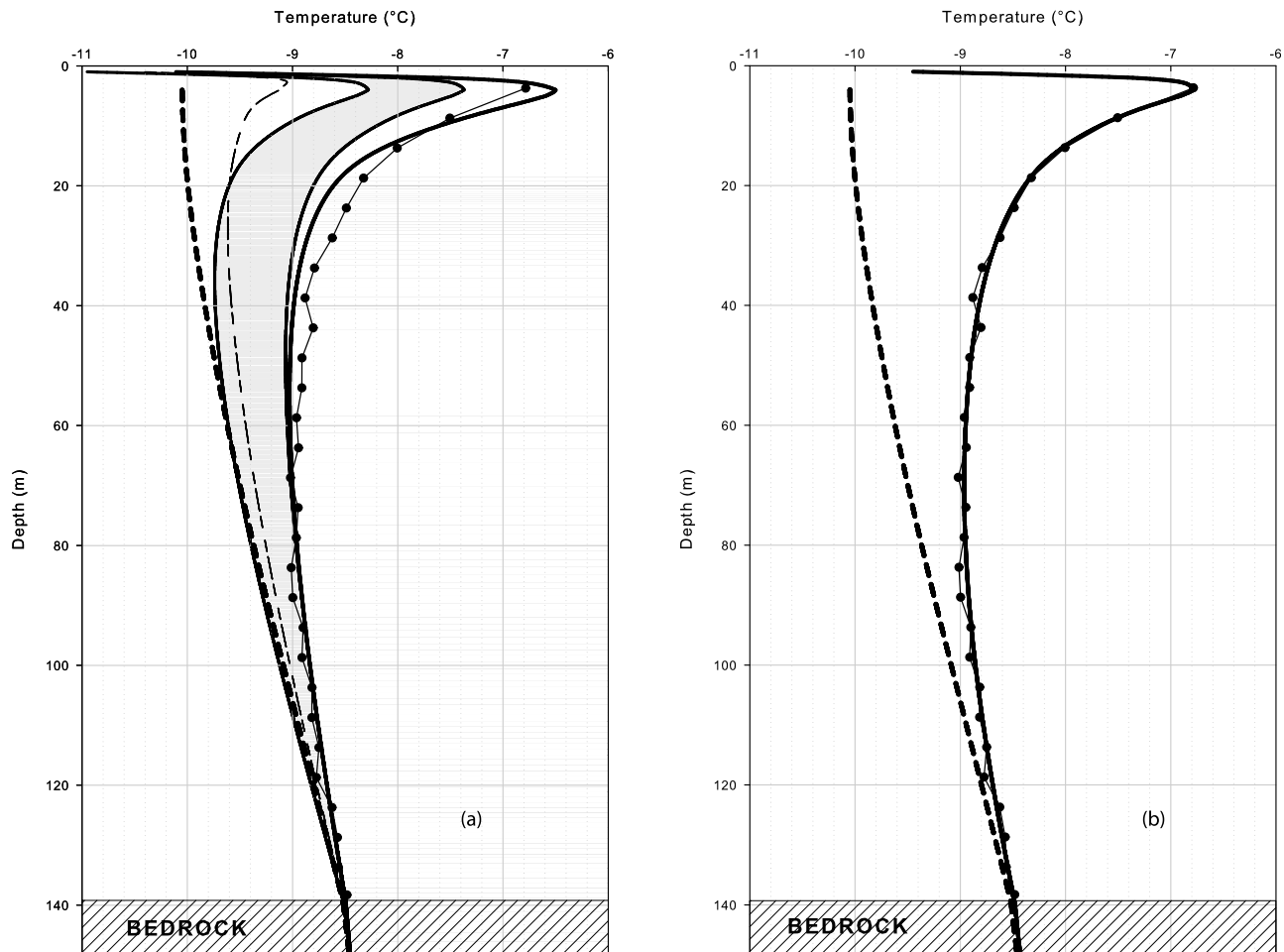
Figure 2. Vertical englacial temperature profile measured at Illimani (6340 m above sea level (asl)) in June 1999 (thin line with black dots). Modeled profile assuming a steady state climate with a constant secular temperature of 263.1 K (dashed line) and a constant geothermal flux of 22 \times 10^{-3} \text{ W m}^{-2} . (a) Modeled temperature profiles assuming a steady state before 1967 and using La Paz air temperature data after 1967 without taking into account the latent heat resulting from surface meltwater refreezing (thin dashed line) and taking into account the latent heat resulting from refreezing (melting factor a = 1.1 \text{ W m}^{-2} \text{ K}^{-1} ) for a geothermal flux varying from 18 to 26 \times 10^{-3} \text{ W m}^{-2} (gray zone) and modeled temperature profile with a forced melting factor a = 1.7 \text{ W m}^{-2} \text{ K}^{-1} (thick line). (b) Modeled temperature profile assuming a steady state before 1900, assuming a 0.4 K warming between 1900 and 1962, and using La Paz air temperature after 1900 with a constant geothermal flux of 22 \times 10^{-3} \text{ W m}^{-2} and a melting factor of 1.1 \text{ W m}^{-2} \text{ K}^{-1} (thick line) (see section 4 for more details).
