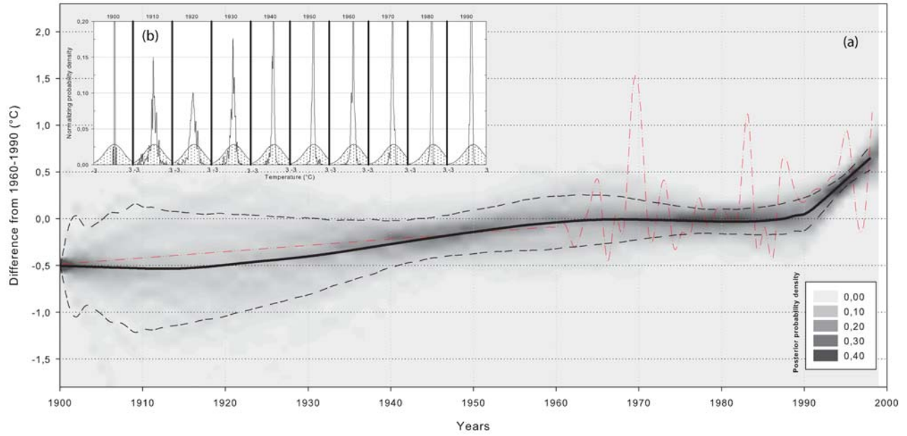
Figure 3. (a) Reconstructed air temperature at Illimani (6340 m asl) over the 20th century using bore-hole temperature profile inversion (thick line) compared with La Paz air temperature (red dashed line after 1962). The two black dashed lines form an envelope corresponding to model uncertainties according to posterior probability density standard deviation. The gray scale represents the past surface temperature probability distribution. (b) Posterior (thin line) and prior (dotted surface) probability density functions of surface temperature each 10 years (see section 5 for more details).
