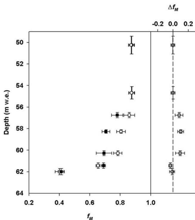
Fig. 3. f_M OC (white) and f_M EC (black) determined in seven sample pairs for Colle Gnifetti (circle: MICADAS CO 2 samples; squares: TANDY graphite samples), together with 1\sigma uncertainty ranges; grey squares mark the difference \Delta f_M ( f_M OC– f_M EC), with the dotted line indicating a perfect match. Error bars on the depth axis describe the depth ranges for the single ice segments.
