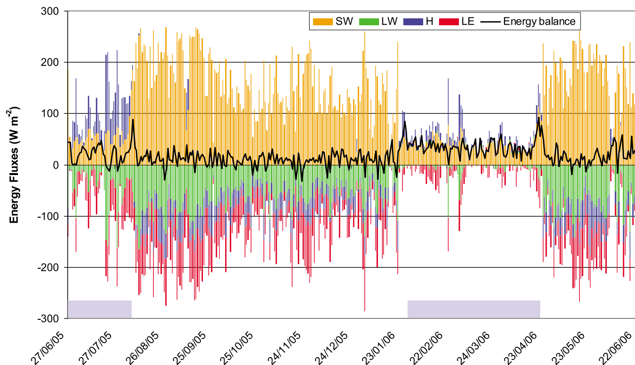
Figure 5. Daily means of net short-wave radiation SW, net long-wave radiation LW, sensible, H , and latent, LE, turbulent fluxes, and the surface energy balance computed with model run 4 parameterization over the entire measurement period at 4860 m asl at the moraine site. Also shown in shaded boxes are the long periods with snow below AWSm.
