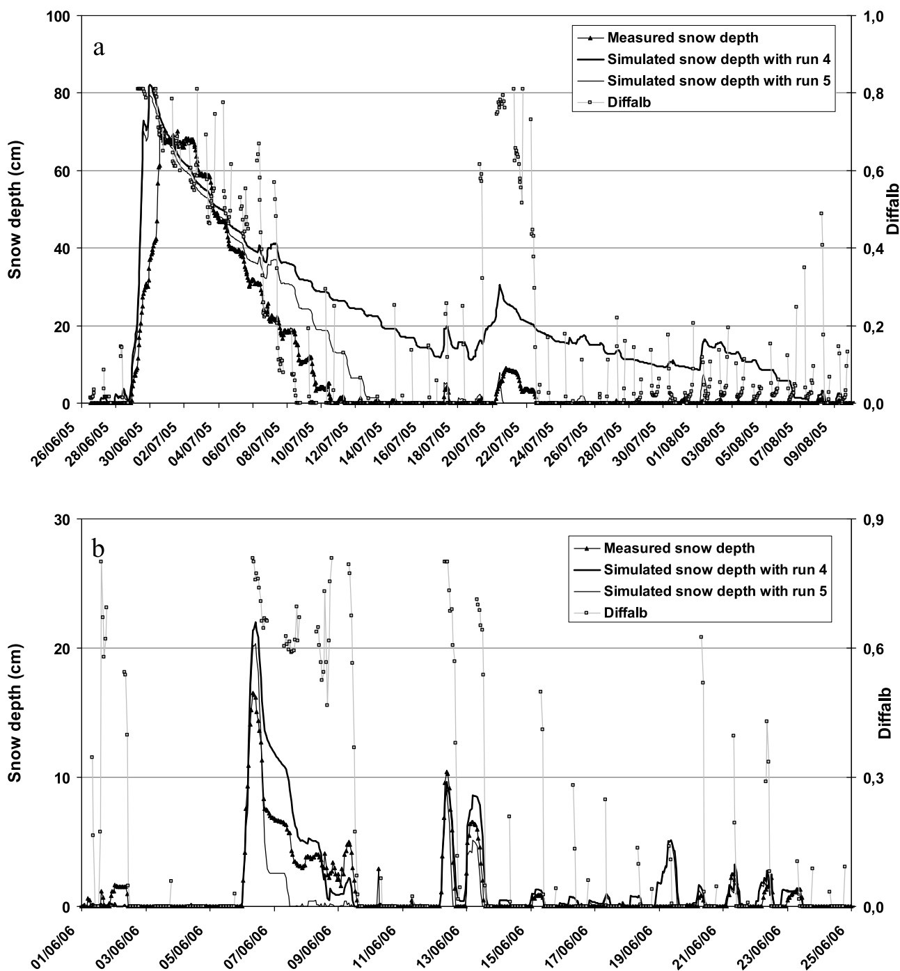
Figure 6. Simulated snow depth from model run 4 (bold line) and model run 5 (solid line) compared to measured snow depth (triangles) for two periods: (a) 26 June–9 August 2005 (heavy snowfall) and (b) 1–25 June 2006 (light snowfall). Also shown is the dimensionless parameter diffalbedo (squares) (diffalbedo = hourly mean albedo – measured bare soil albedo).
