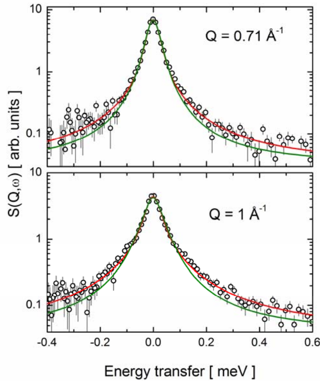
Figure 6. The low-resolution QENS spectra measured for the Na-hectorite sample. Lines: (green) fit by model 16, (red) fit by model 17.
