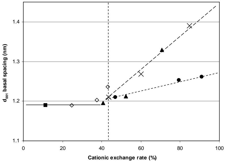
FIG. 7: Variation of the d_{001} basal spacing at 50% of relative humidity of the \text{NH}_4 -SWy-2 sample after 7 days interaction with water (black rectangle), acetic acid (open diamond), formic acid (black triangle), chloroacetic acid (cross) and oxalic acid (black circle) versus the cationic exchange rate calculated from \text{NH}_4^+ concentration. Lines are trends for the eyes.
