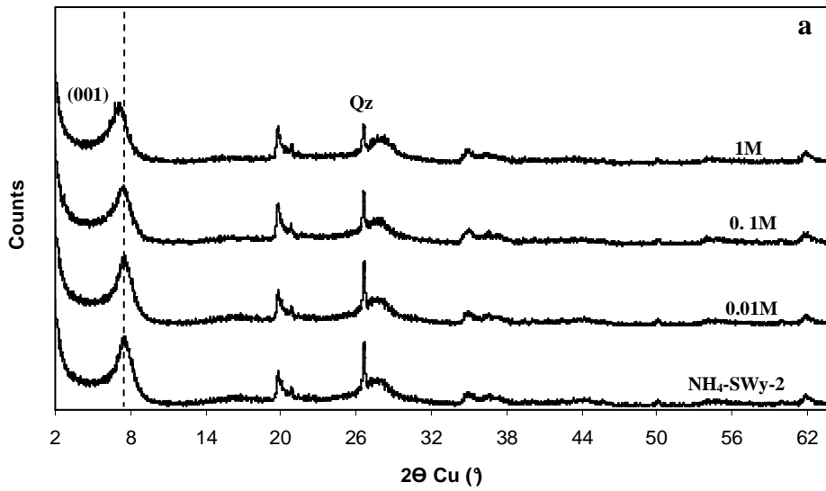
FIG. 3: XRD patterns of NH 4 smectite interacted with water used as reference, acetic acid (a), formic acid (b), chloroacetic acid (c) and oxalic acid (d). Acids are in 0.01, 0.1 and 1M concentration. Qz indicates the presence of quartz.
